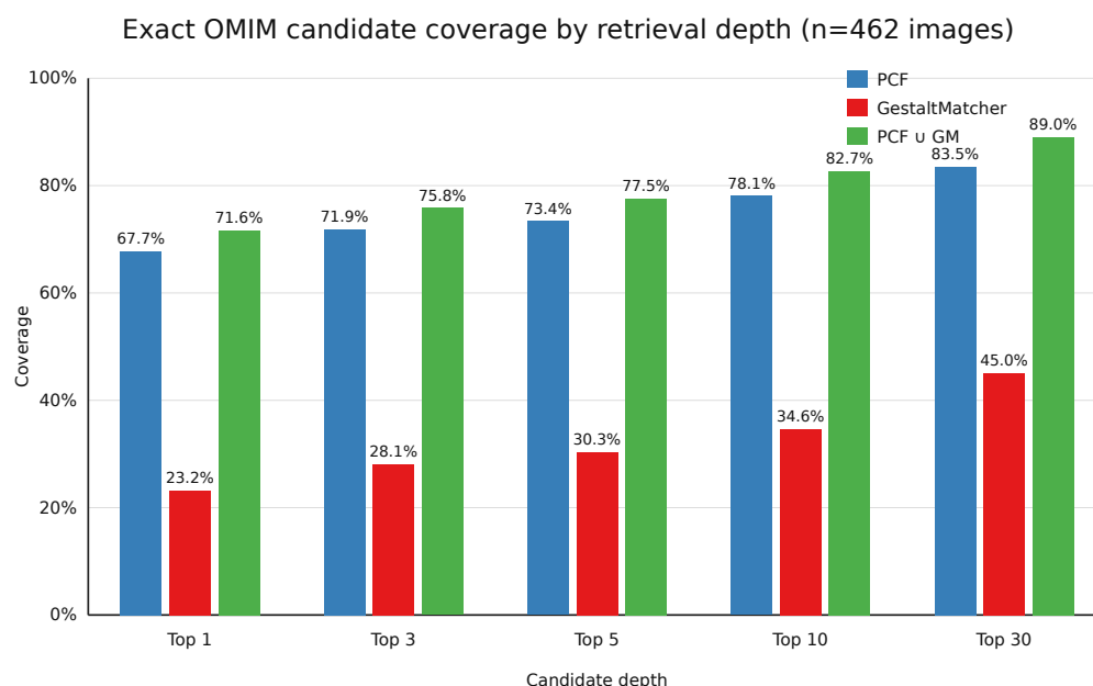
Figure 7: Deeper specialist rankings expose candidates hidden by a fixed top-five input limit. Exact OMIM inclusion was evaluated for 462 facial-image instances linked to 368 patients across 54 disorders. Bars show candidate coverage for PubCaseFinder (PCF), GestaltMatcher (GM) and their combined lists after duplicate diseases were removed at increasing retrieval depths. Coverage increased from 77.5% at top five to 89.0% at top 30. This figure characterizes the candidate set available before ZebraSeek integration; it is not an end-to-end diagnostic-performance comparison.
