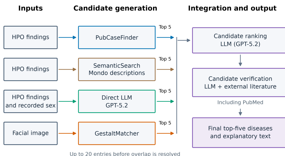
Figure 2: ZebraSeek workflow. Facial images are analyzed by GestaltMatcher; HPO terms are supplied to PubCaseFinder and SemanticSearch; and HPO terms together with recorded sex are supplied to the direct LLM component. Each component provides up to five candidates. LLM-based ranking and literature-based verification produce a final top-five list with explanatory text.
