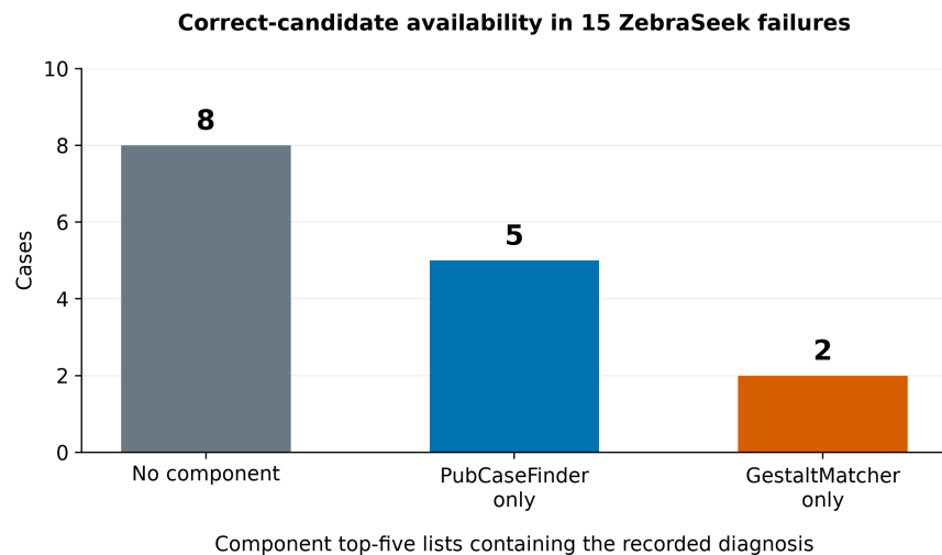
Figure 6: Correct-candidate availability among the 15 ZebraSeek failures at rank five. Eight cases had no correct candidate in any component's top-five list. Five had a correct candidate only in PubCaseFinder and two only in GestaltMatcher. The latter seven cases distinguish failure to retain an available diagnosis from absence of that diagnosis in all initial lists.
