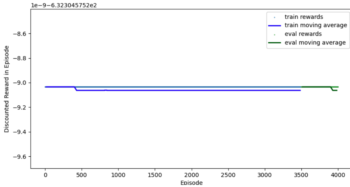
Figure 2: Value Iterations
