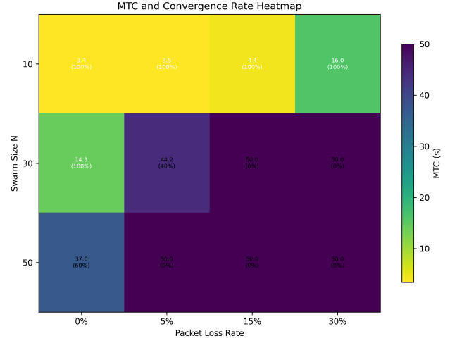
Fig. 4. Mean MTC over swarm size \times packet loss, annotated with convergence rate. The jump toward the cap traces the synchronization–staleness phase transition of Thm. 1(ii).
