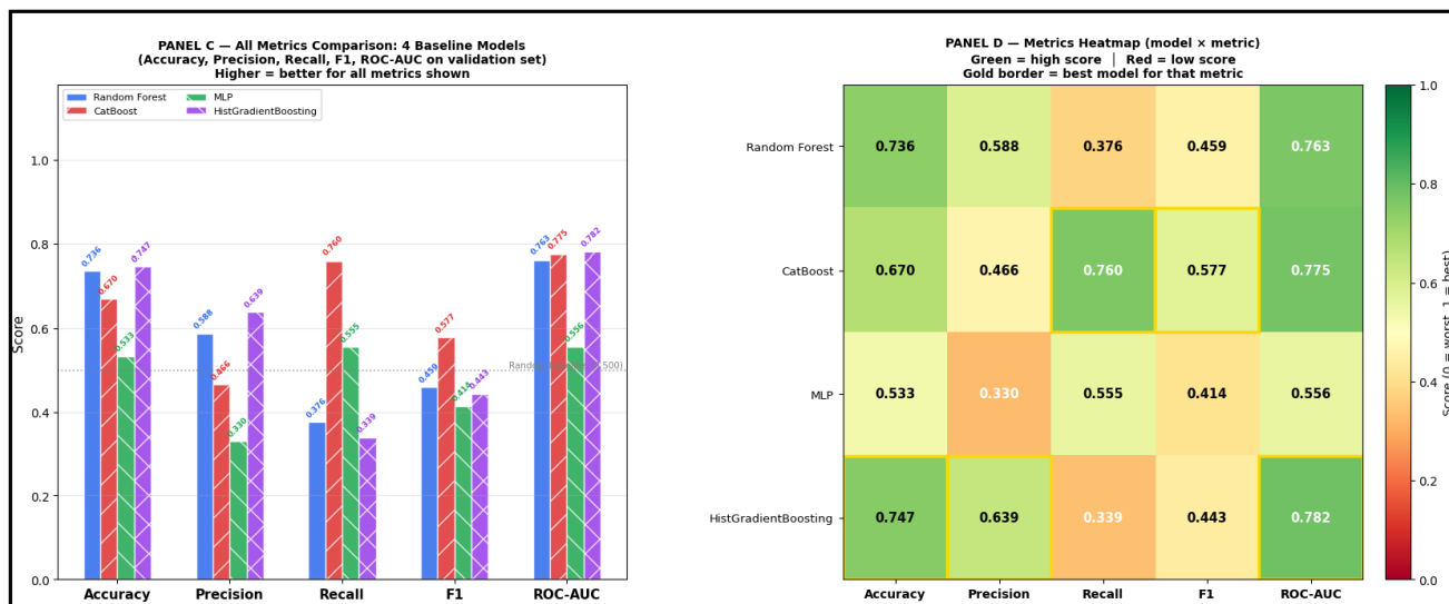
FIG 7: ALL METRICS COMPARISON AND HEATMAP FOR BASELINE MODELS
