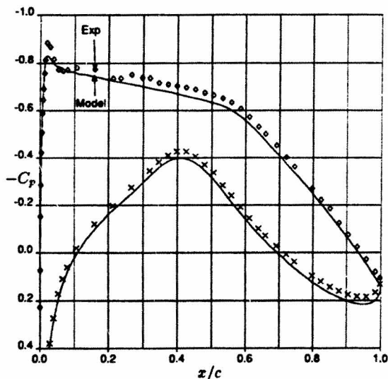
Figure 20: Pressure distribution for Case 1, blunt RAE 2822 airfoil.
