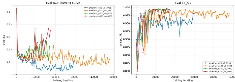
Figure 1: Held-out validation curves for the four small ER sizes. Left: validation BCE (lower is better). Right: approximation ratio pp-AR (higher is better).
