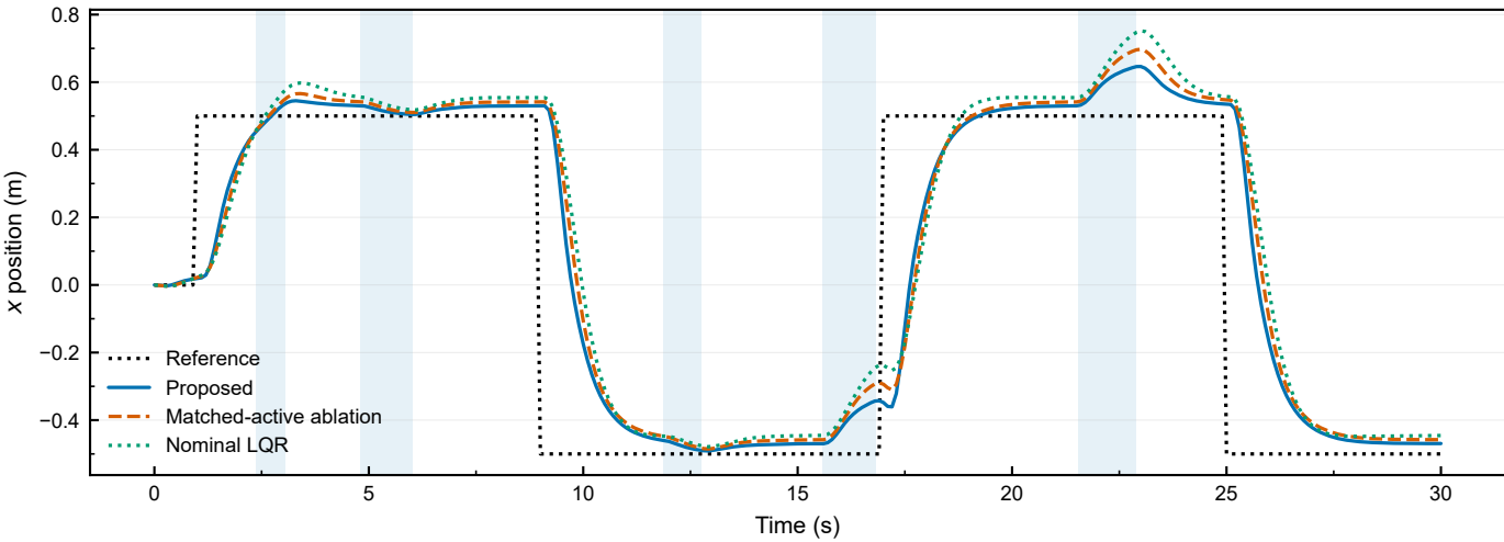
Position tracking along x under multi-gust disturbance
