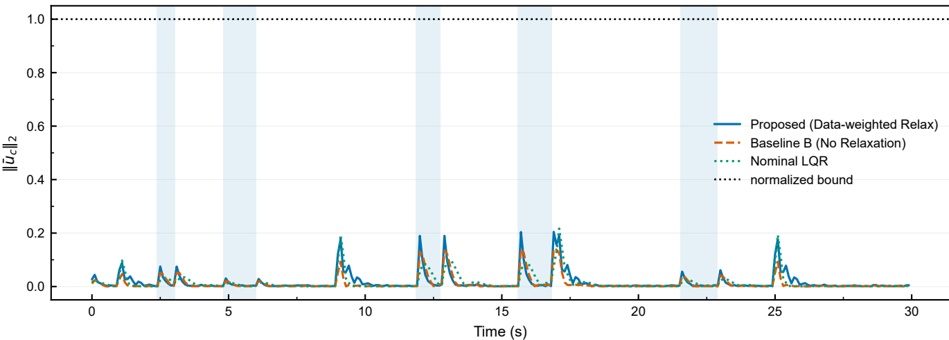
Increment command norm (rate constraint activity)
