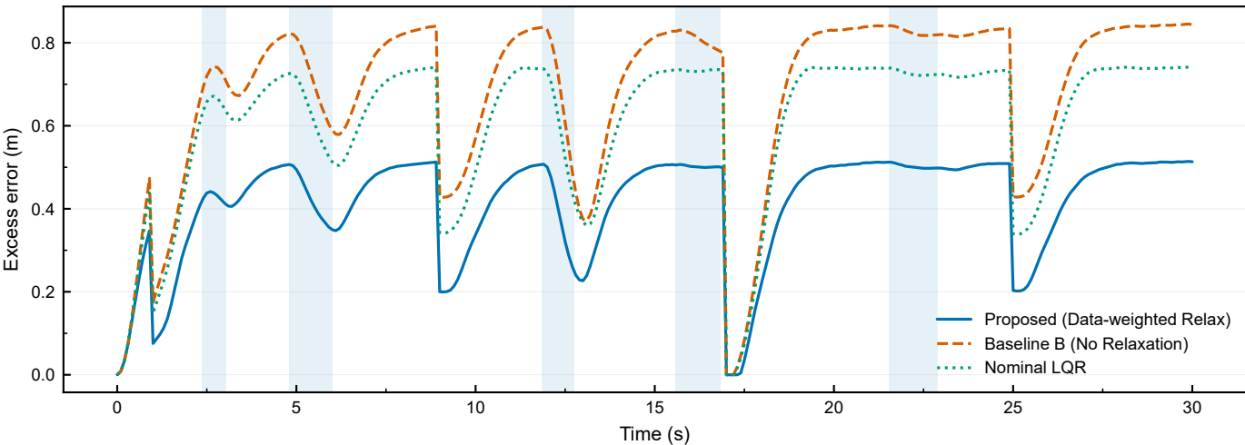
Disturbance-induced excess tracking error
