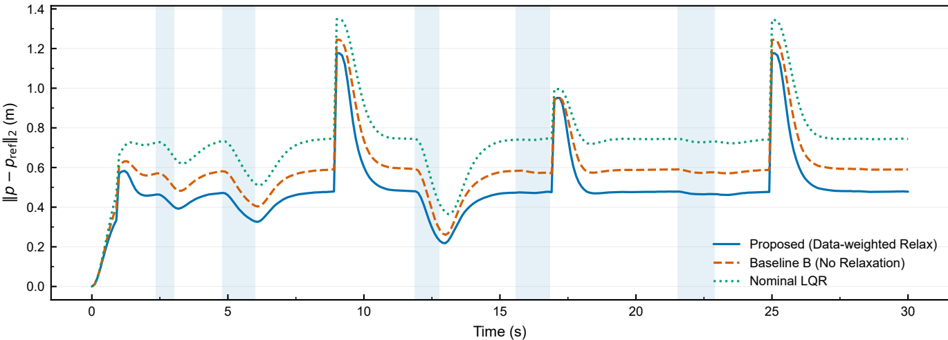
Position tracking error norm (disturbed)
