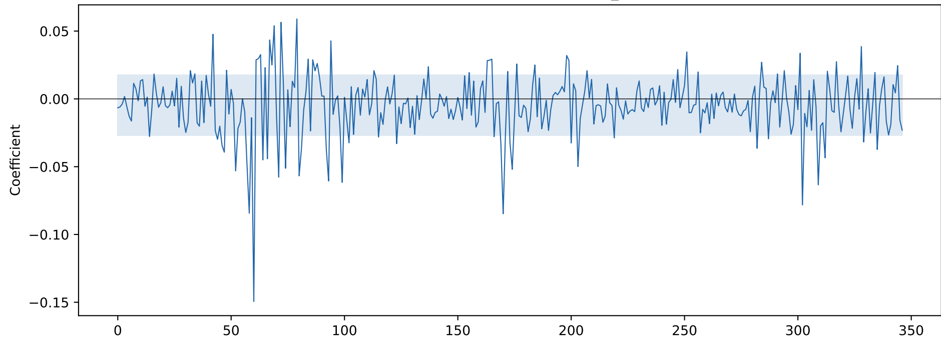
ACF of \beta_{\Delta G} Series
