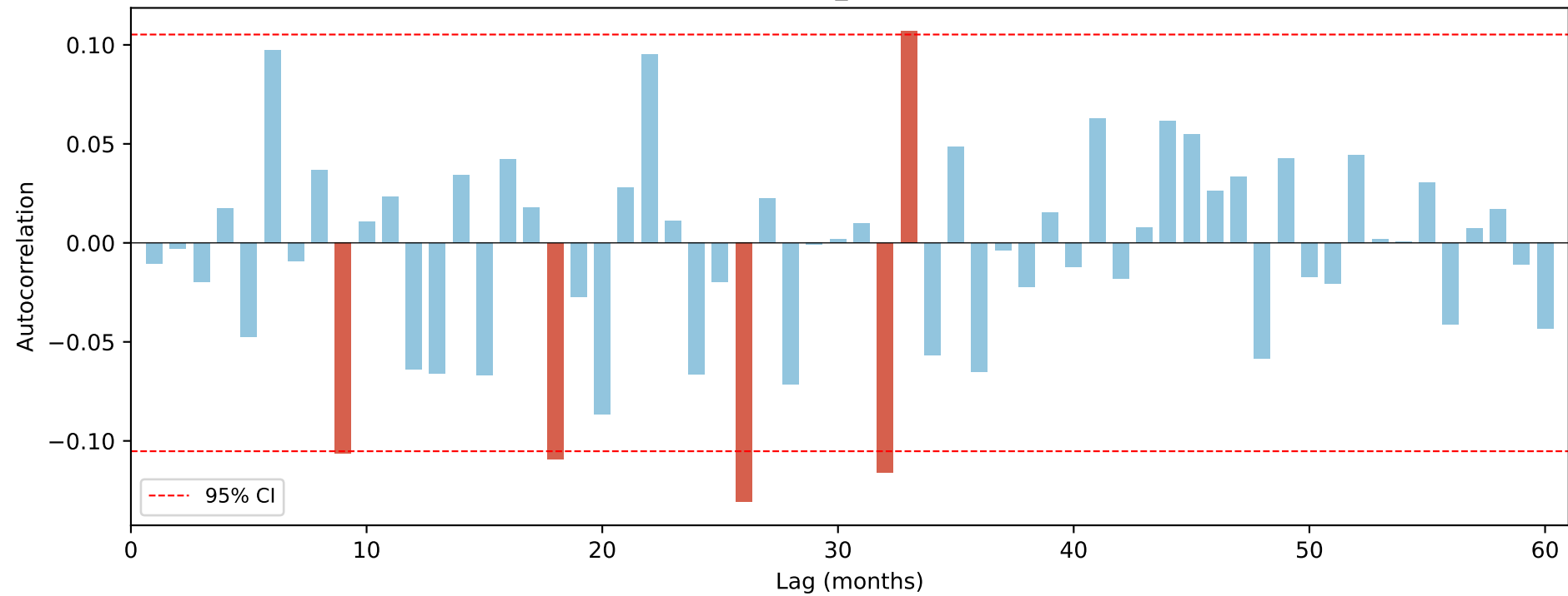
ACF of \beta_{\Delta G} Series
