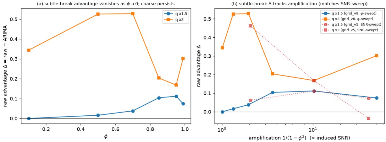
Figure 2. The \varphi \times q cross-grid ( grid_v8_phiqbreak ). Left: raw's advantage \Delta = \text{detect}(\text{raw}) - \text{detect}(\text{ARIMA}) against \varphi ; the subtle \times 1.5 advantage vanishes at \varphi = 0.1 and peaks at \varphi = 0.95 , while the coarse \times 3 advantage persists at every \varphi . Right: the same \Delta against the 1/(1-\varphi^2) amplification factor, with the fixed- \varphi SNR-sweep values ( grid_v5 ) overlaid — on the subtle break the \varphi -swept and SNR-swept experiments coincide at matched induced SNR; note the \Delta values are differences between near-floor detection rates.
