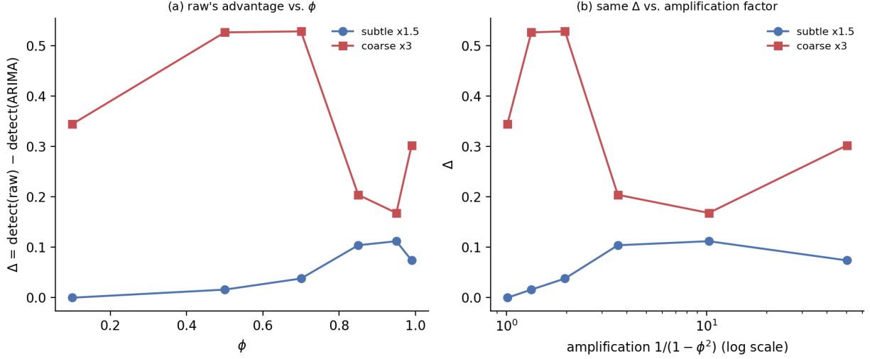
Figure 2. The \phi \times q cross-grid (grid_v8_phiqb). Left: raw's advantage \Delta = \text{detect}(\text{raw}) - \text{detect}(\text{ARIMA}) against \phi ; the subtle \times 1.5 advantage vanishes at \phi = 0.1 and peaks at \phi = 0.95 , while the coarse \times 3 advantage persists at every \phi . Right: the same \Delta against the 1/(1 - \phi^2) amplification factor, with the fixed- \phi SNR-sweep values (grid_v5) overlaid — on the subtle break the \phi -swept and SNR-swept experiments coincide at matched induced SNR; note the \Delta values are differences between near-floor detection rates.
