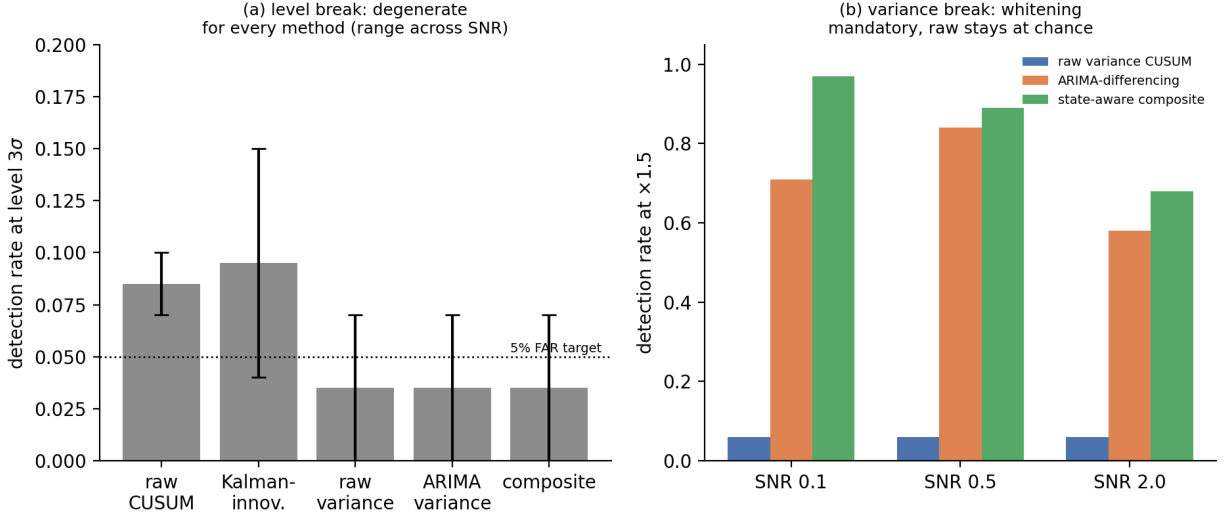
Figure 3. The local-level (random-walk state) arena at SNR 0.5 ( grid_v7_1level ). Left: a 3\sigma level break is degenerate for every method — all five detectors sit at the 5% FAR line. Right: a \times 1.5 observation-noise variance break is caught by both whitened detectors — ARIMA-differencing (0.84) and the state-aware composite (0.89, a distinct, broader statistic, not the same CUSUM re-run on Kalman innovations) — while the raw variance CUSUM stays at chance: whitening is mandatory once Y is nonstationary.
