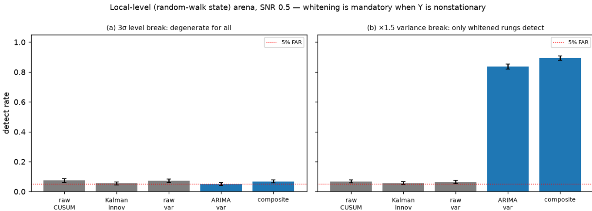
Figure 3. The local-level (random-walk state) arena at SNR 0.5 ( grid_v7_l1level ). Left: a 3\sigma level break is degenerate for every method — all five detectors sit at the 5% FAR line. Right: a \times 1.5 observation-noise variance break is caught only by the whitened rungs (ARIMA-differencing 0.84, Kalman composite 0.89) while the raw variance CUSUM stays at chance — whitening is mandatory once Y is nonstationary.
