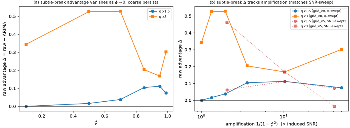
Figure 2. The \phi \times q cross-grid (grid_v8_phiqbreak). Left: raw’s advantage \Delta = \text{detect}(\text{raw}) - \text{detect}(\text{ARIMA}) against \phi ; the subtle \times 1.5 advantage vanishes at \phi = 0.1 and peaks at \phi = 0.95 , while the coarse \times 3 advantage persists at every \phi . Right: the same \Delta against the 1/(1 - \phi^2) amplification factor, with the fixed- \phi SNR-sweep values (grid_v5) overlaid — on the subtle break the \phi -swept and SNR-swept experiments coincide at matched induced SNR; note the \Delta values are differences between near-floor detection rates.
