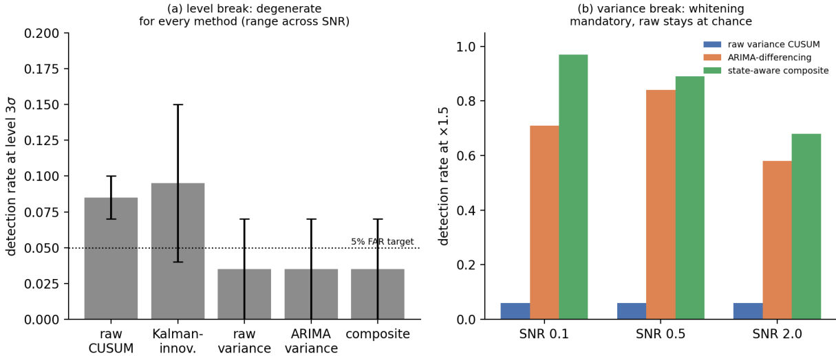
Figure 3. The local-level (random-walk state) arena at SNR 0.5 (grid_v7_1level). Left: a 3\sigma level break is degenerate for every method — all five detectors sit at the 5% FAR line. Right: a \times 1.5 observation-noise variance break is caught by both whitened detectors — ARIMA-differencing (0.84) and the state-aware composite (0.89, a distinct, broader statistic, not the same CUSUM re-run on Kalman innovations) — while the raw variance CUSUM stays at chance: whitening is mandatory once Y is nonstationary.
