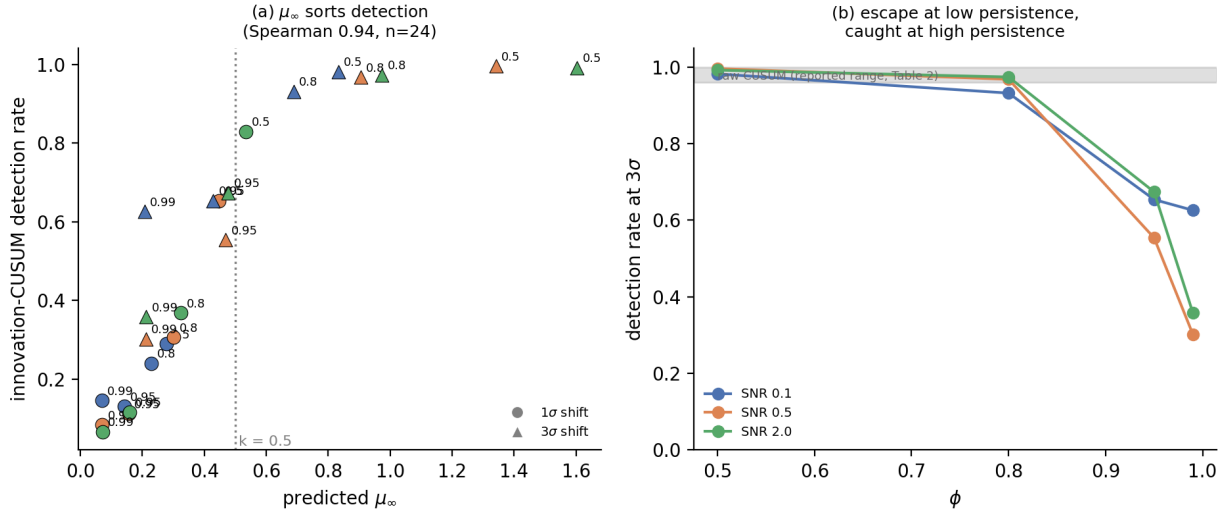
Figure 1. The \varphi sweep (grid_v6_phisweep). Left: predicted asymptotic innovation drift \mu_\infty against the observed innovation-CUSUM detection rate for every \varphi \times \text{SNR} \times \text{shift} cell (point labels = \varphi ); \mu_\infty sorts detection (Spearman 0.94), and the dotted line marks the fast-or-never boundary k = 0.5 . Right: at 3\sigma the detector escapes the trap at low persistence (0.97–1.00 at \varphi = 0.5 –0.8) and is caught at high persistence (0.30–0.67 at \varphi = 0.95 –0.99).
