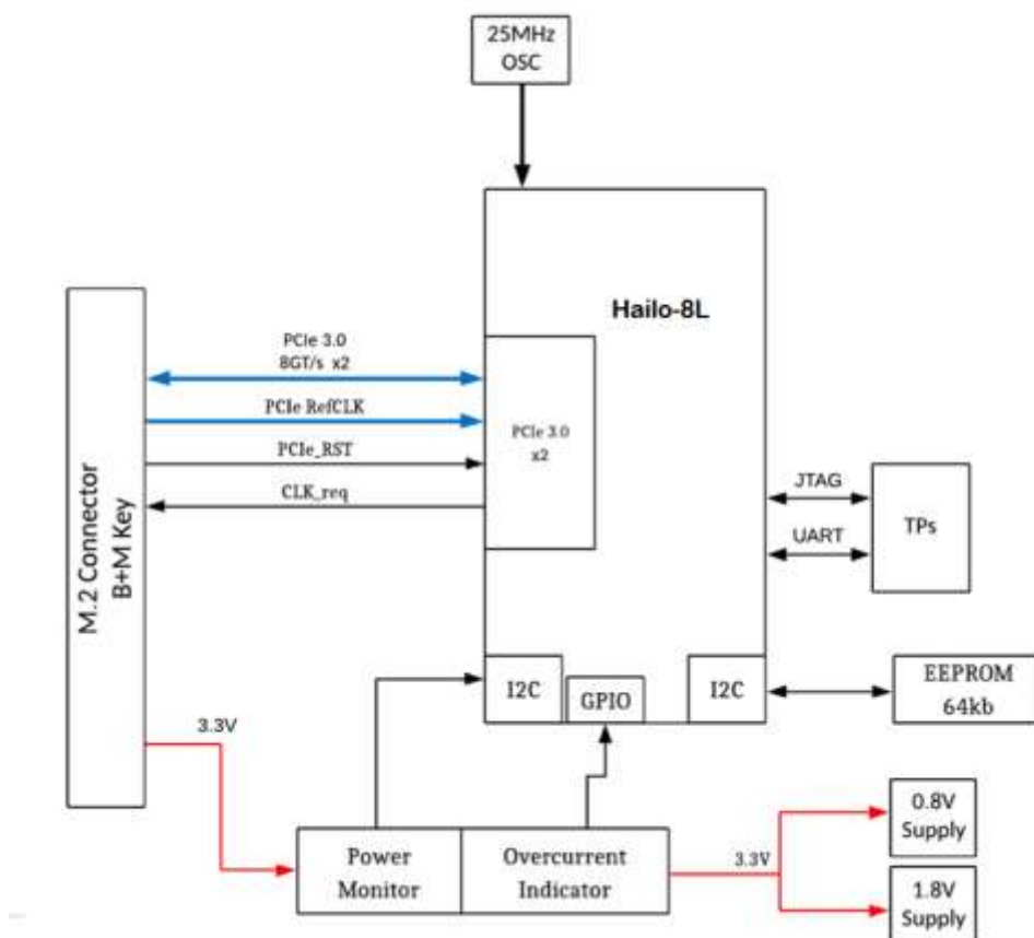
Figure 1: Hailo-8L M.2 Key B+M ET Functional block Diagram
