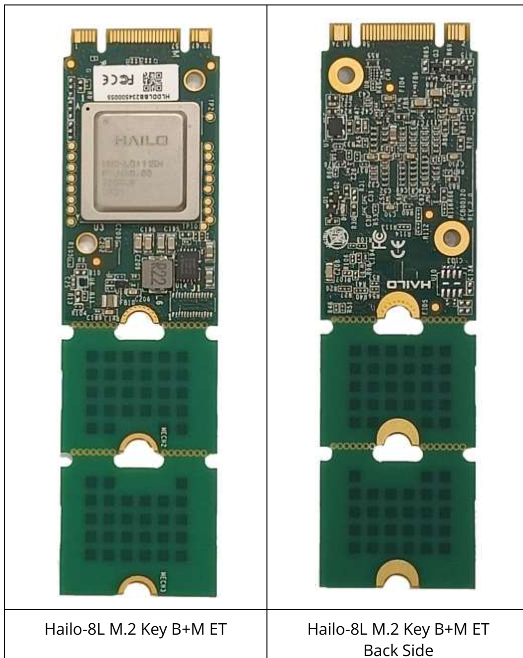
Figure 3: Module board layout for Hailo-8L M.2 Key B+M ET.
