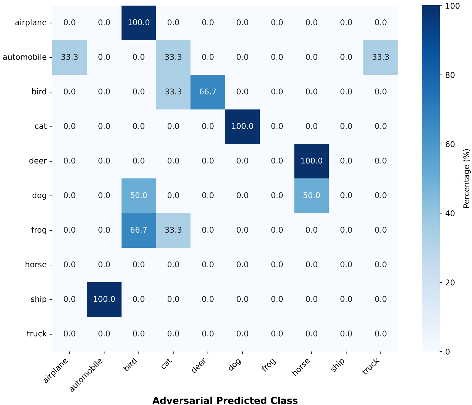
SparseFool Confusion Matrix (% of successful attacks per class)
