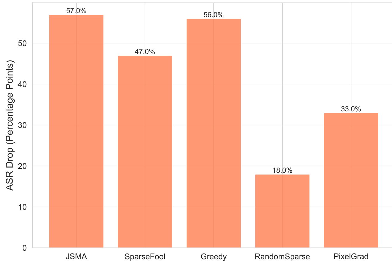
Absolute ASR Drop on Defended Model
