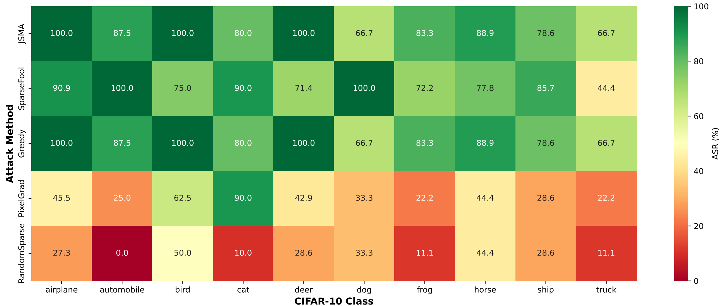
Class-Specific Attack Success Rate (ResNet18)
