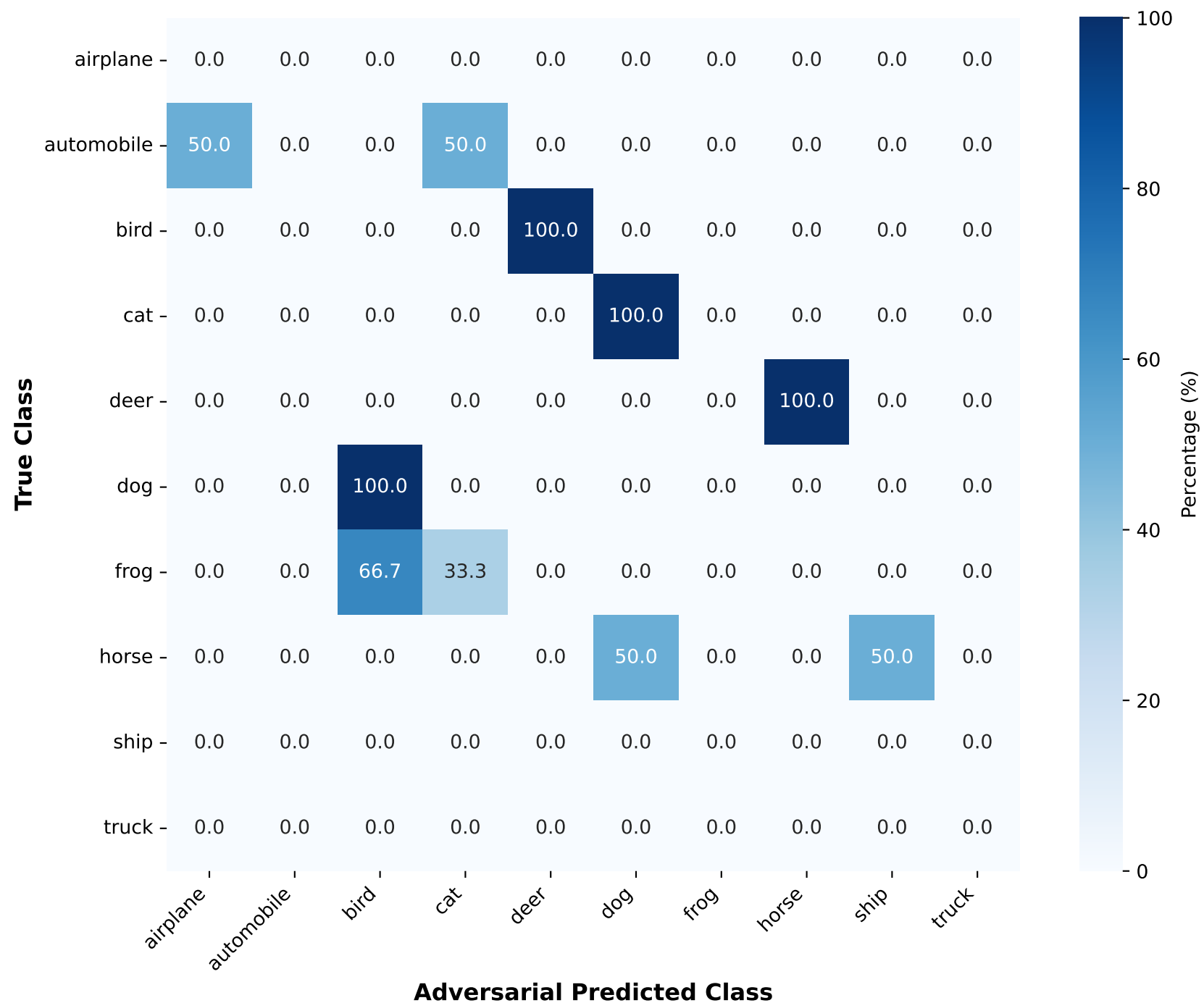
Greedy Confusion Matrix (% of successful attacks per class)
