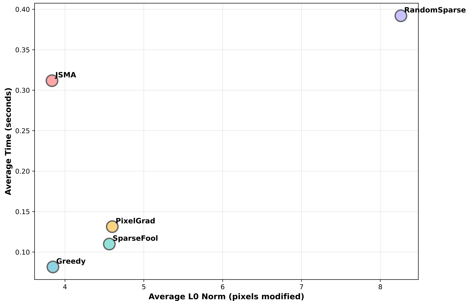
Sparsity vs Computational Cost
