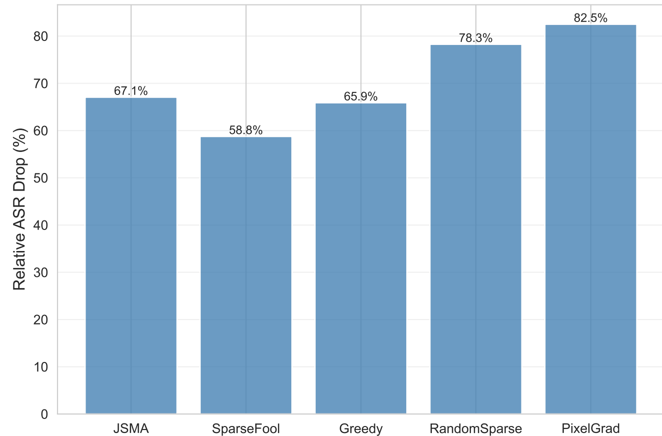
Relative ASR Drop on Defended Model
