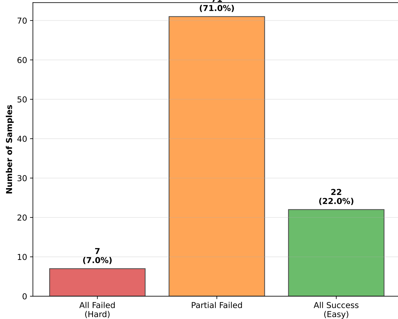
Sample Classification by Attack Difficulty
