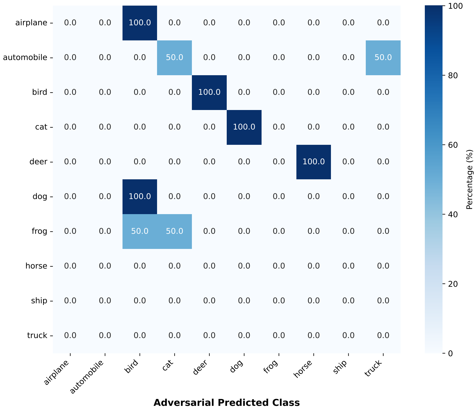
RandomSparse Confusion Matrix (% of successful attacks per class)
