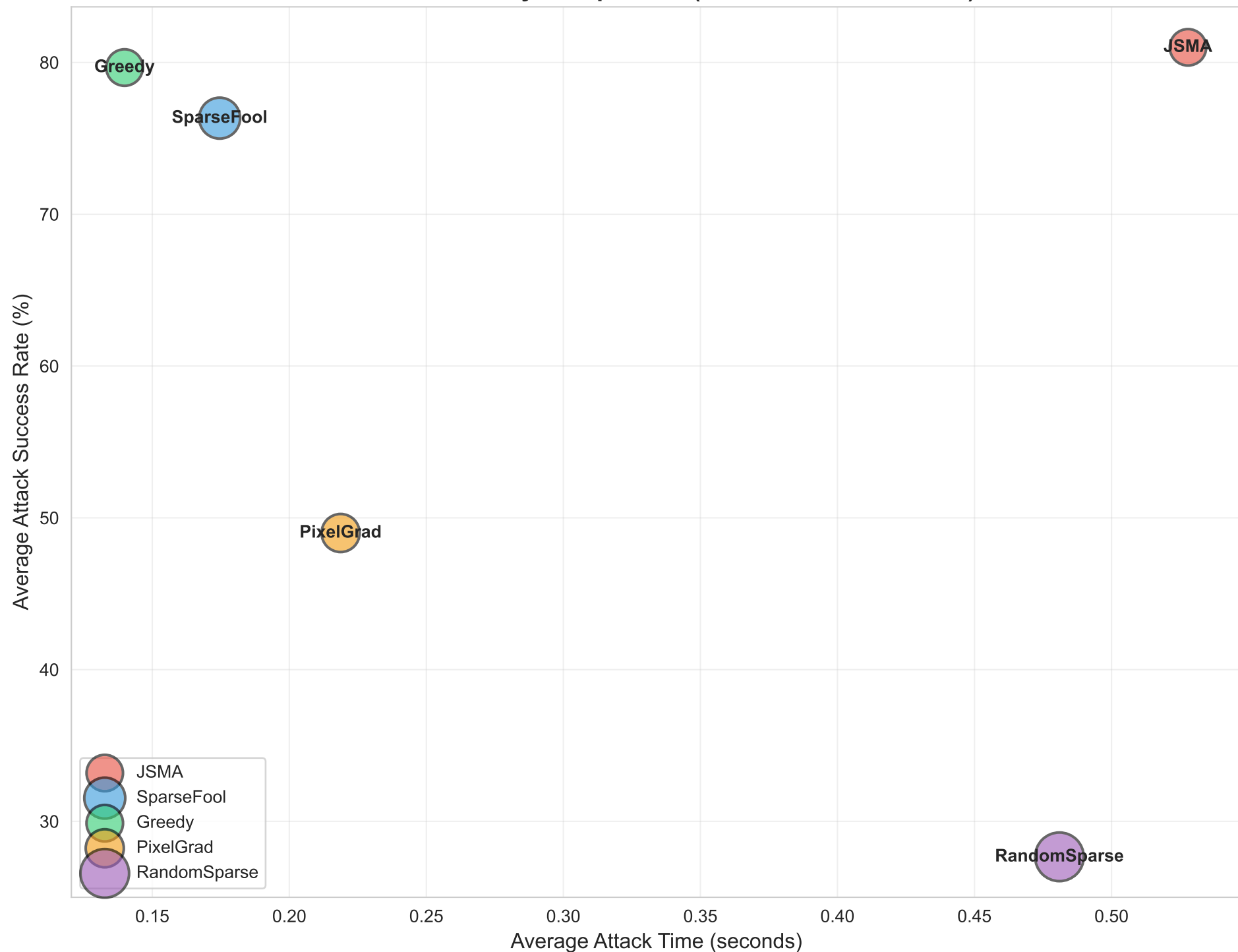
Attack Efficiency Comparison (Bubble Size = L0 Norm)
