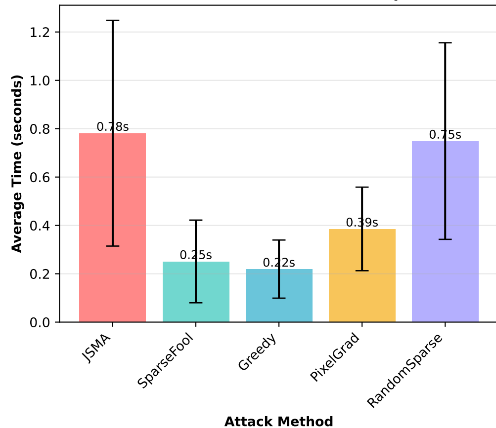
MOBILENETV2 - Attack Time Comparison
