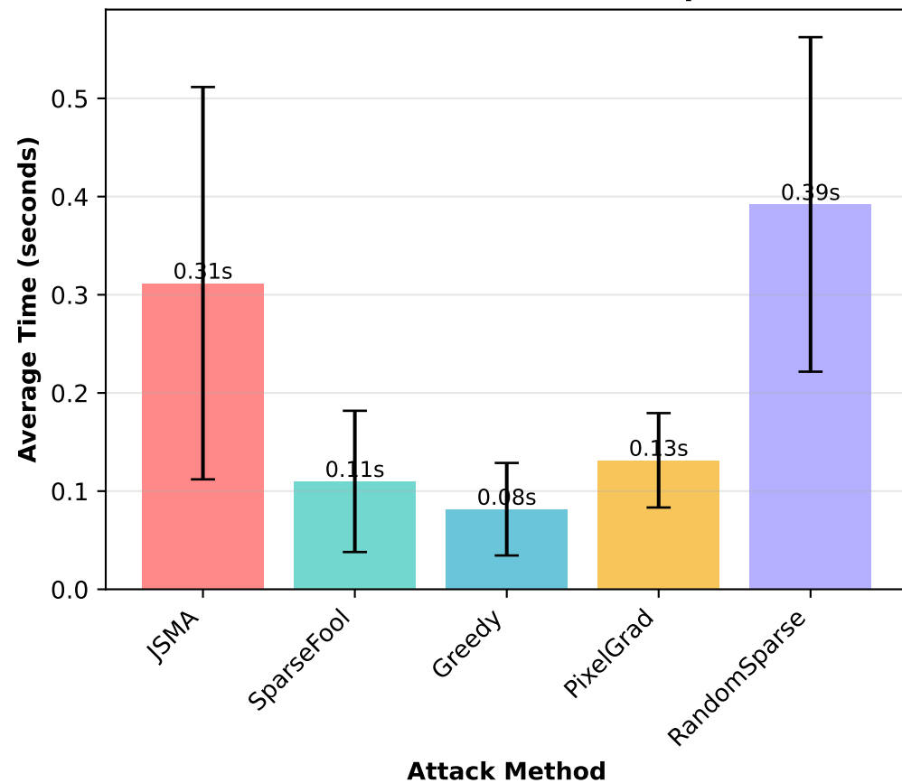
RESNET18 - Attack Time Comparison
