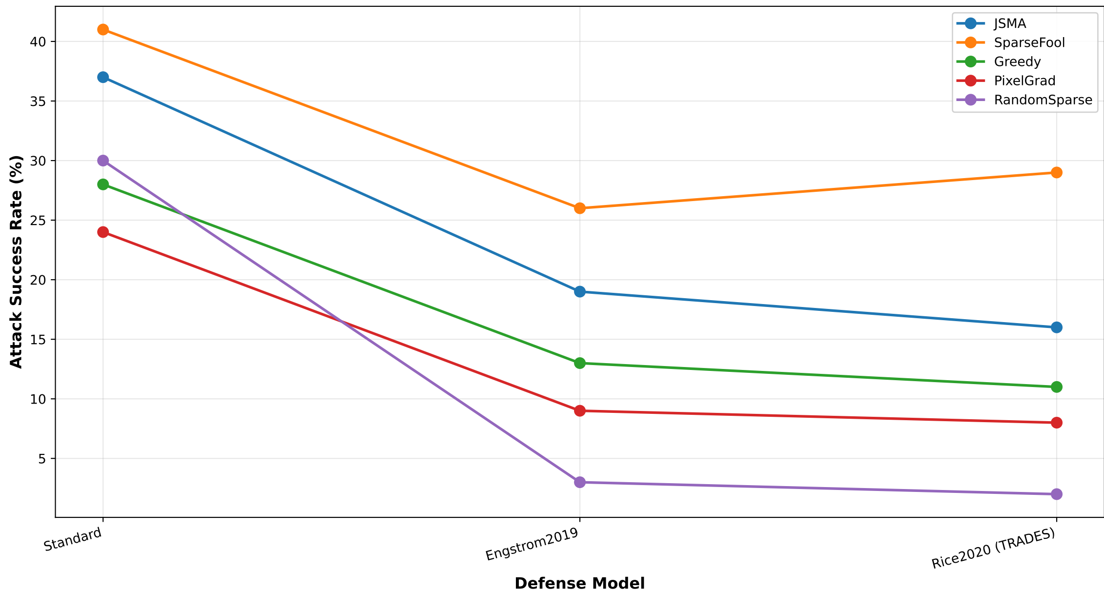
Method Robustness: ASR Decline Across Defense Levels
