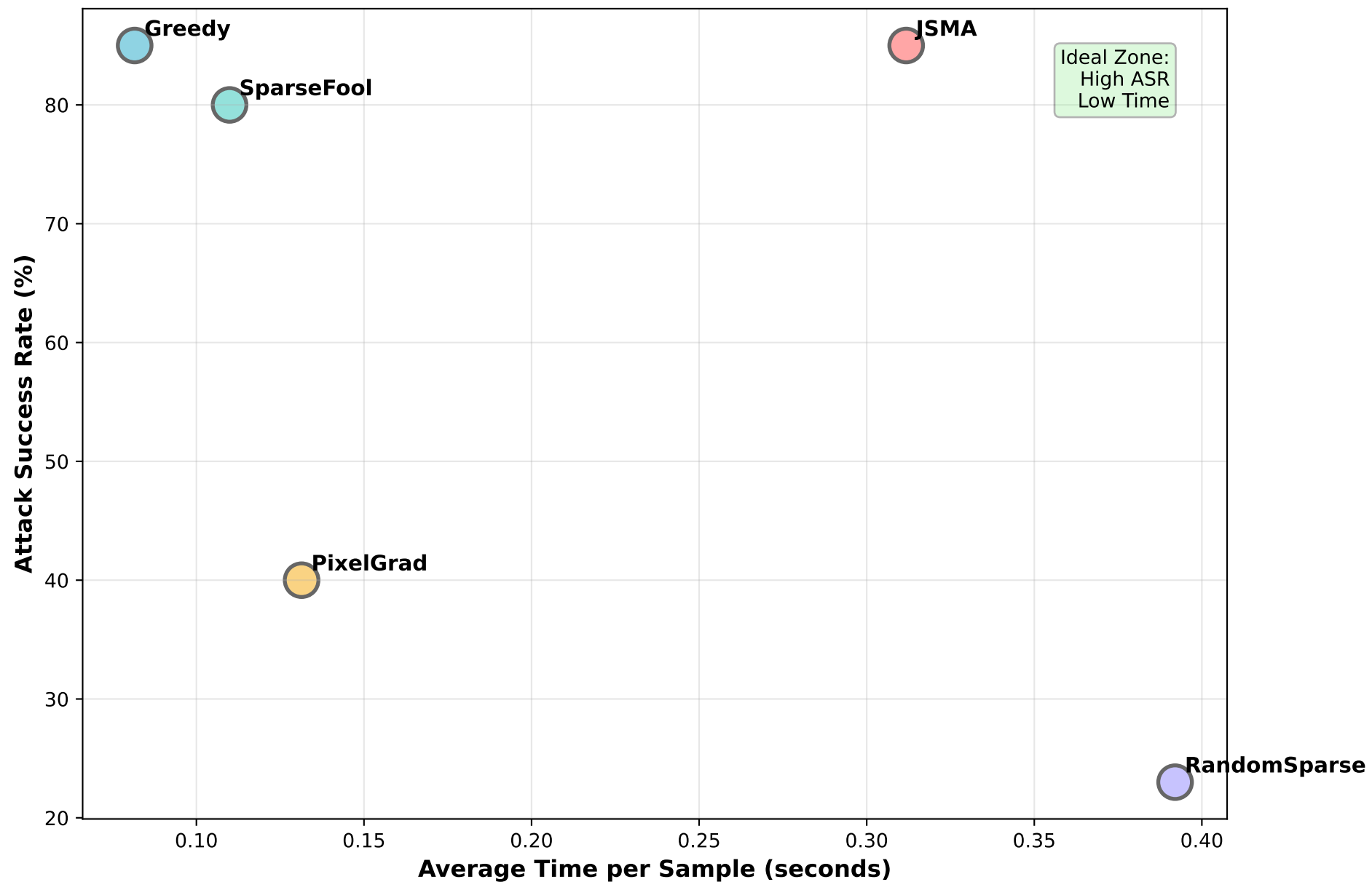
Attack Efficiency Trade-off: ASR vs Time
