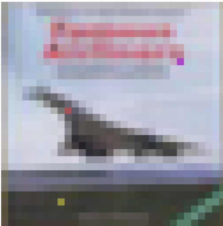
SparseFool → bird
