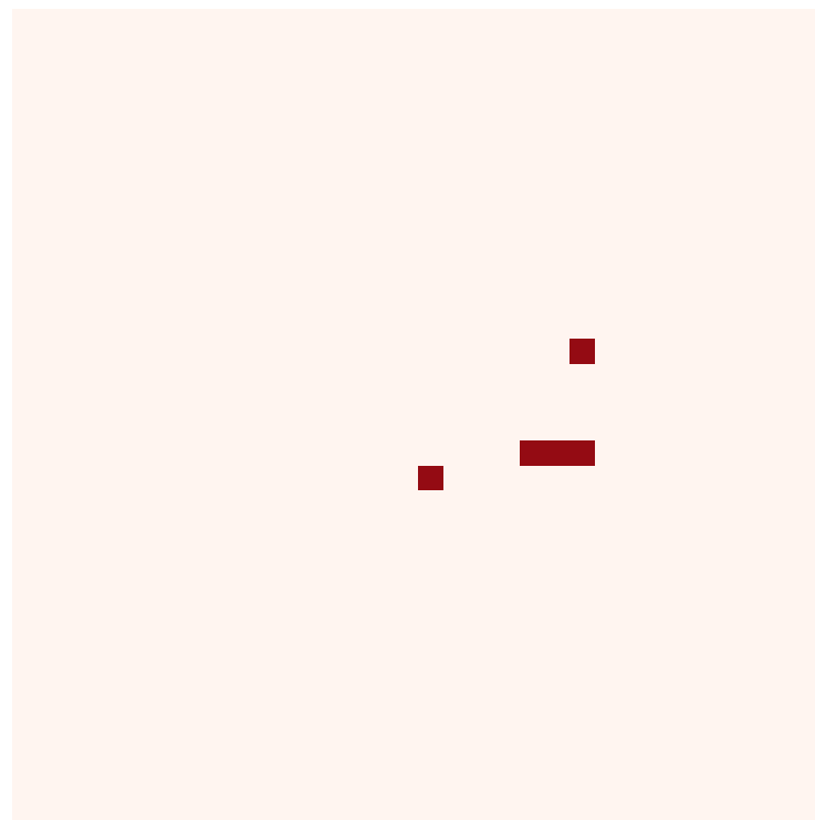
Greedy 5 pixels
