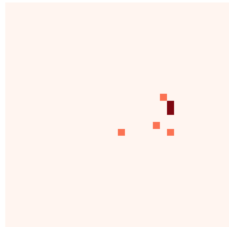
SparseFool 8 pixels
