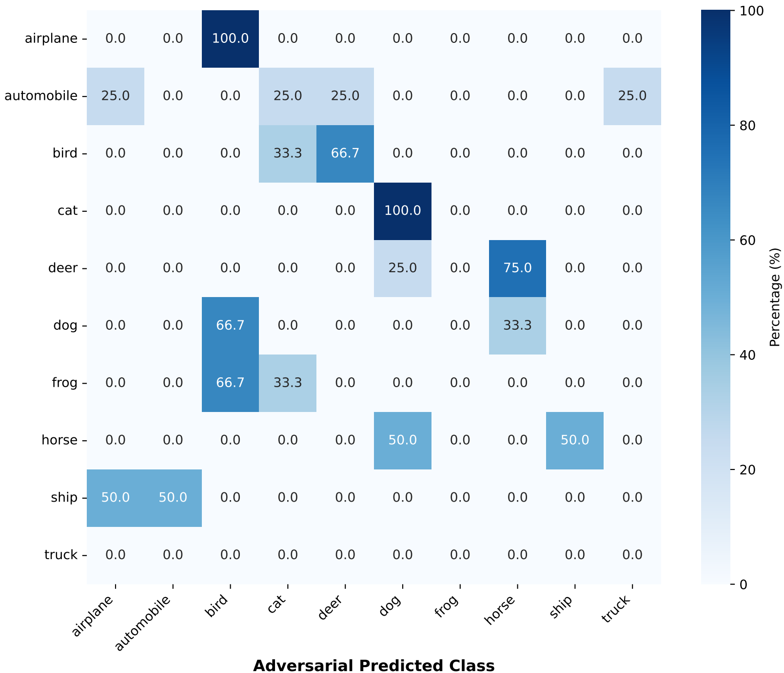
JSMA Confusion Matrix (% of successful attacks per class)
