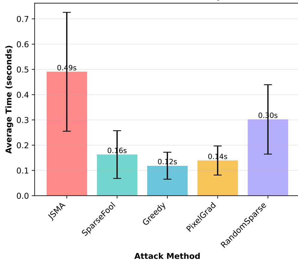
VGG16 - Attack Time Comparison
