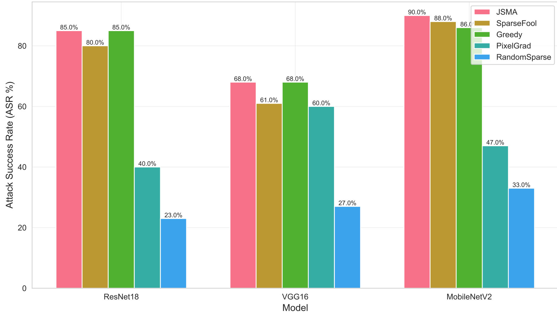
ASR Comparison of 5 Sparse Attack Methods
