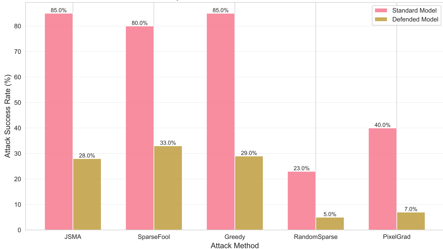
ASR Comparison: Standard vs Defended Model
