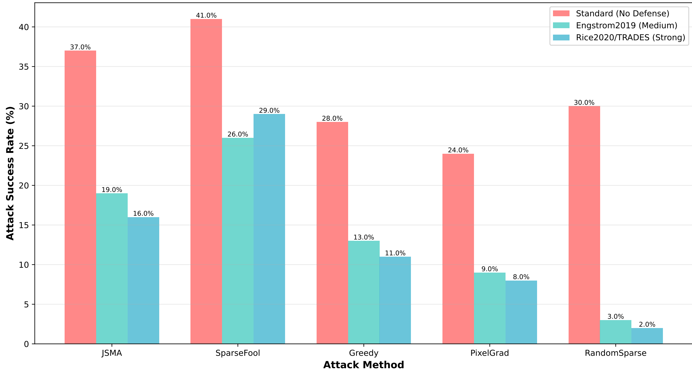
Defense Strength Gradient: ASR Across Three Defense Levels
