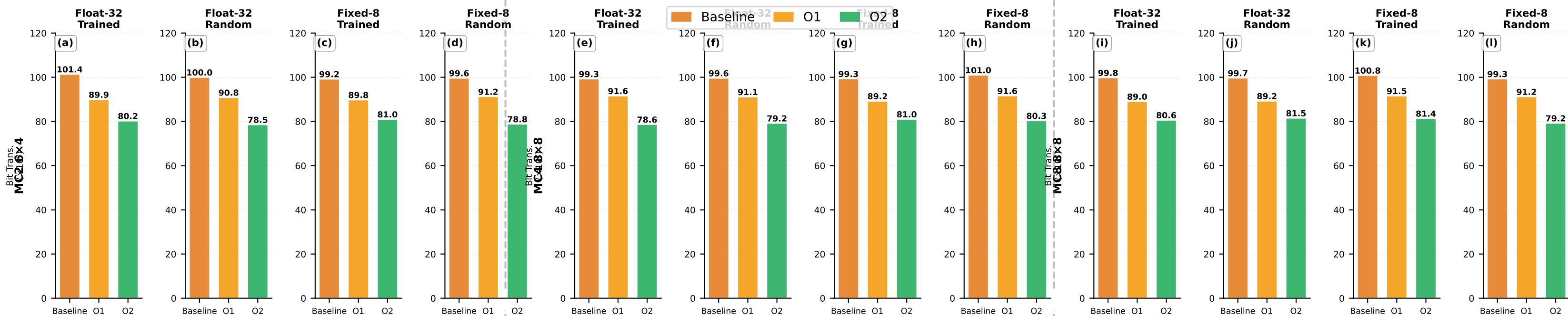
LeNet Model
