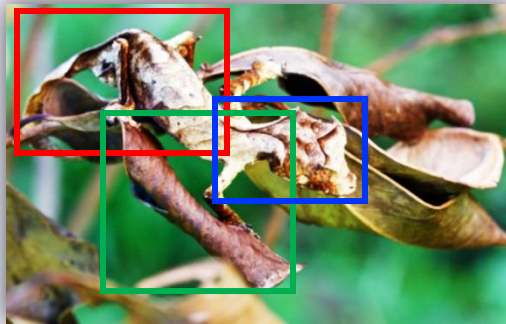
Image + Proposals
