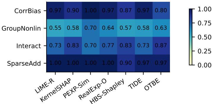
Top-k recovery by scenario
