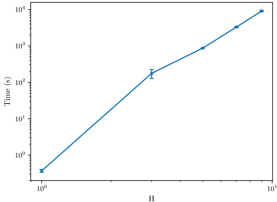
Execution time vs Horizon
