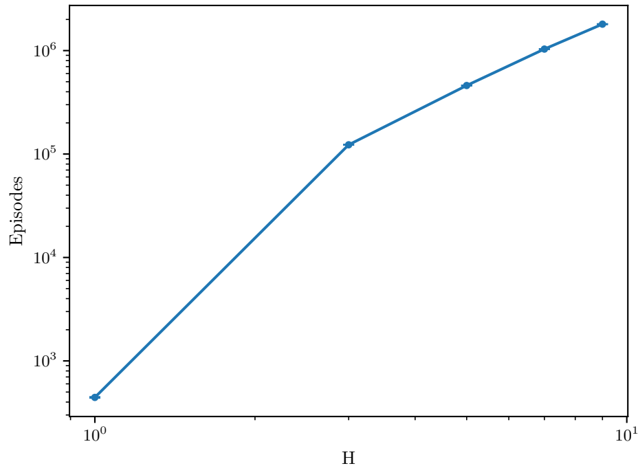
Episodes vs Horizon
