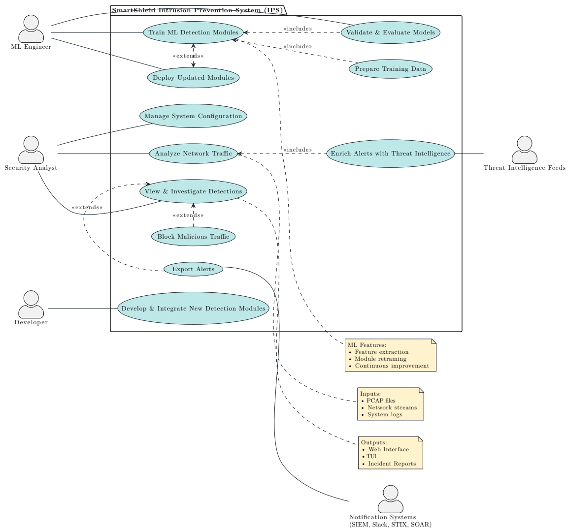
Figure 2.2: Use Case Diagram
