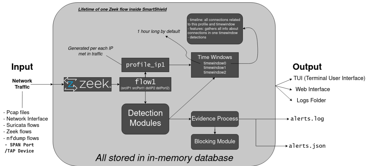
Figure 2.3: SmartShield Architecture
