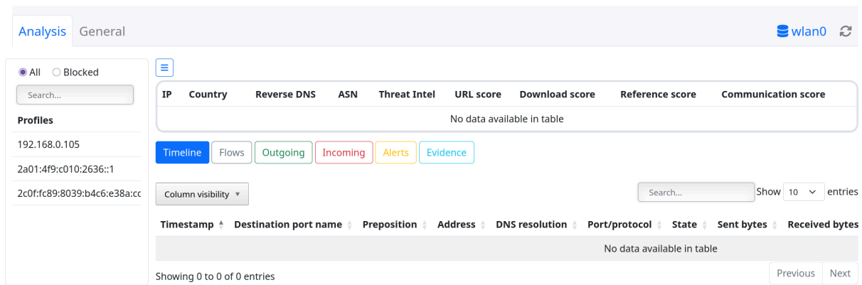
Figure 2.10: Web Interface
