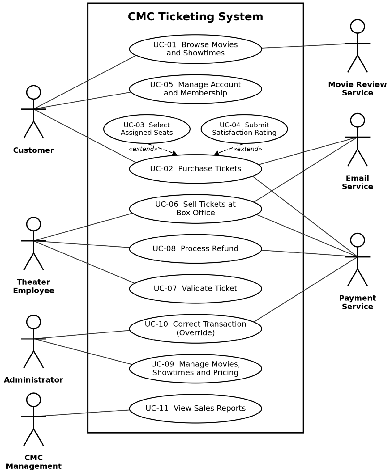
Figure 1. Use-case diagram for the CMC Ticketing System
