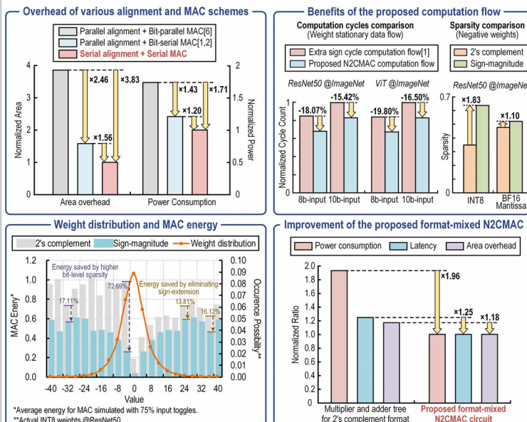
Figure 14.3.5: Proposed CIM macro simulated performance.
