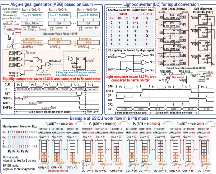
Figure 14.3.3: The ESICU structure for the embedded 2b-serial alignment, ASG for control signal generation, LC for input conversion (top). An example of ESICU workflow in BF16 mode (bottom).
