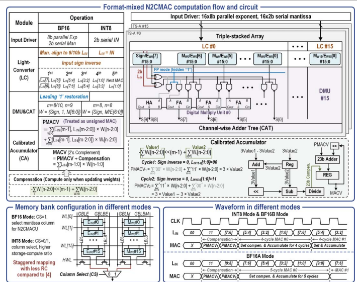
Figure 14.3.4: Detailed implementation of format-mixed N2CMAC computation (top). Memory bank configuration and MAC operation waveforms for 3 computation modes (bottom).
