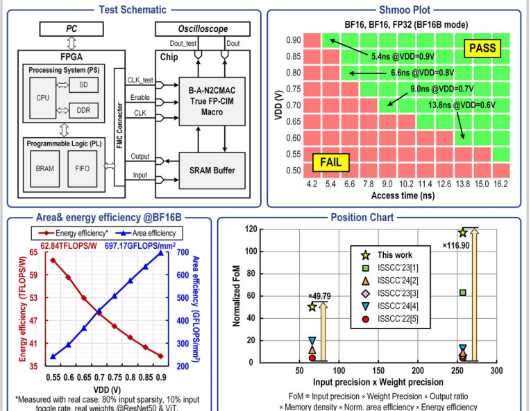
Figure 14.3.6: Measurement results and FoM comparison to prior work.
