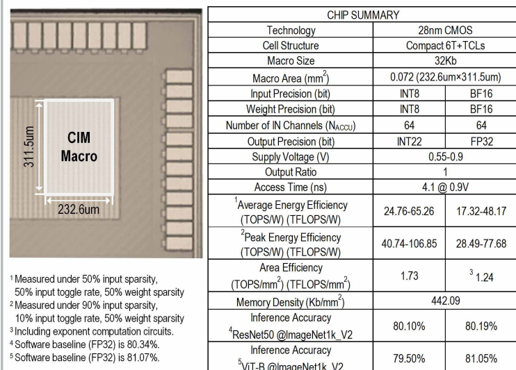
Figure 30.4.7: Die micrograph and summary of key performance metrics.
