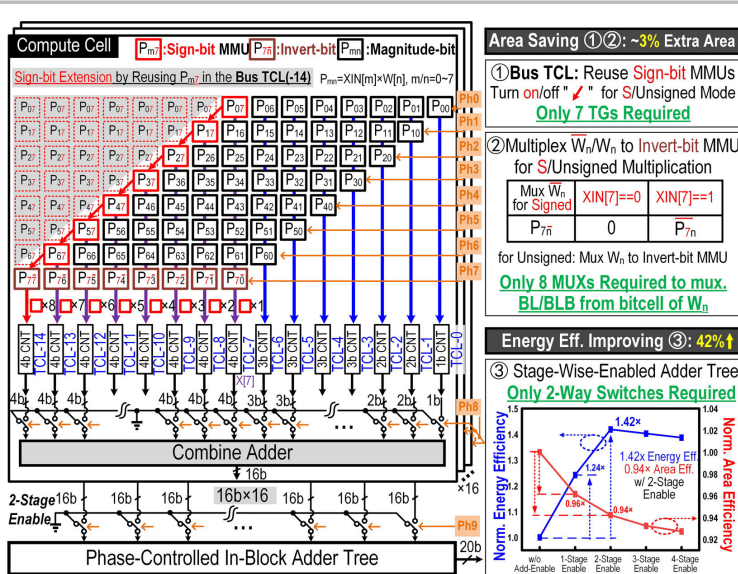
Figure 30.4.4: Embedded sign-bit extension in bus TCL-14 and the enabling-circuit structure for Combine Adder and In-Block Adder Tree.
