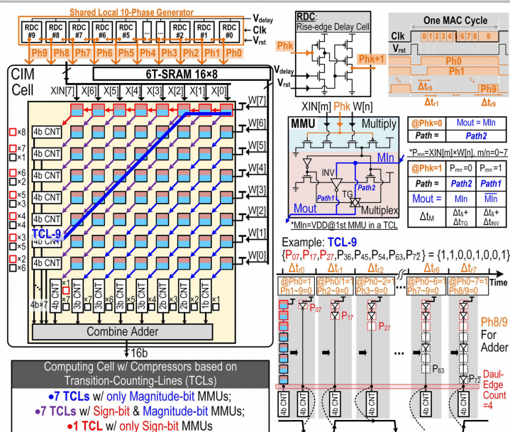
Figure 30.4.3: The structures and workflows of the TCL and the 10-phase generator.
