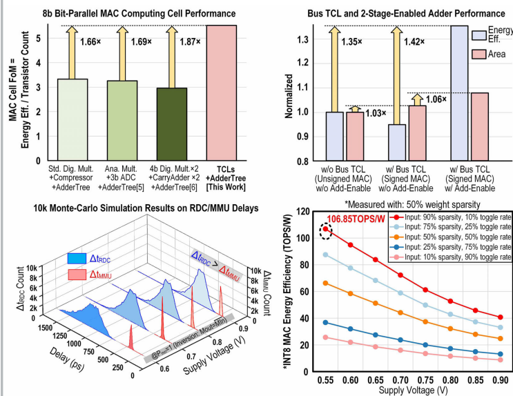
Figure 30.4.5: Simulated MAC computing cell performance and measured energy efficiencies of the proposed CIM macro.
