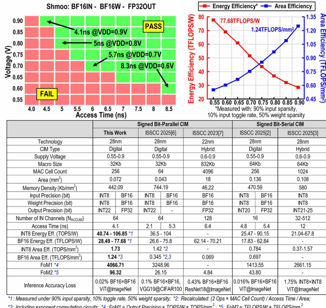
Figure 30.4.6: Measurement results and comparison table.
