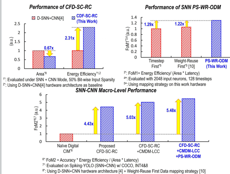
Figure 30.8.5: Simulated performance of proposed schemes.
