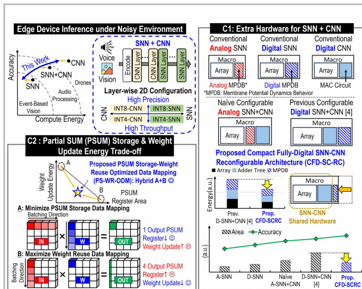
Figure 30.8.1: Motivation and challenges for hybrid SNN-CNN SRAM-CIM.
