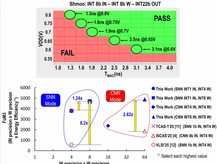
Figure 30.8.6: Measurement results and position chart.
