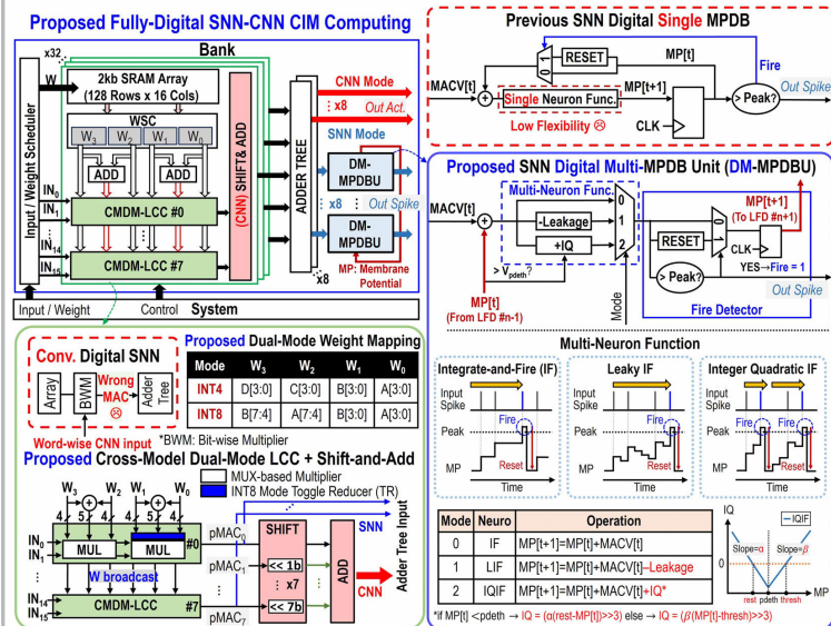
Figure 30.8.3: CDM-LCC and DM-MPDBU structure and operation.
