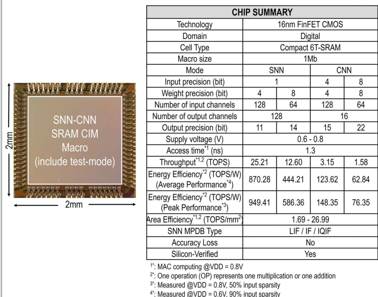
Figure 30.8.7: Die micrograph and performance summary table.
