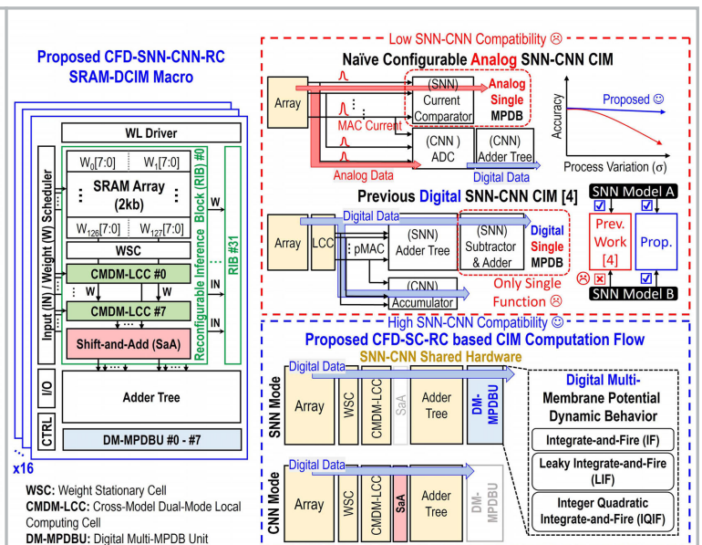
Figure 30.8.2: Structure of proposed SRAM-DCIM macro and CFD-SC-RC operation.
