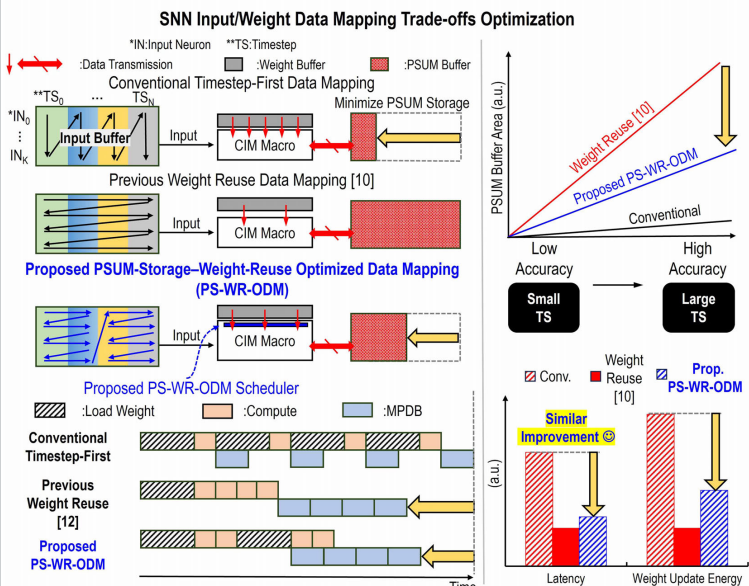
Figure 30.8.4: PS-WR-ODM operational concept.
