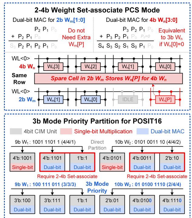
Fig. 9. CPCS with 2-4b weight association and 3b priority partition.
