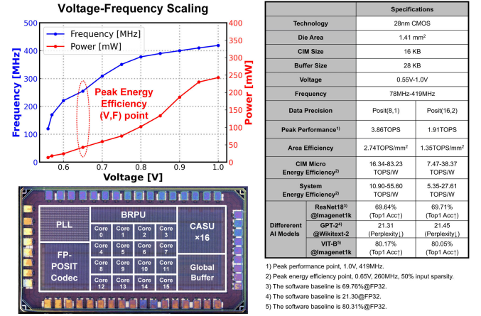
Fig. 14. Chip micrograph and summary of the proposed PD-CIM.
