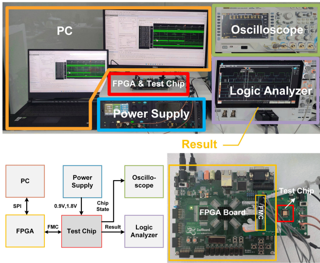
Fig. 16. Verification system of the proposed PD-CIM.
