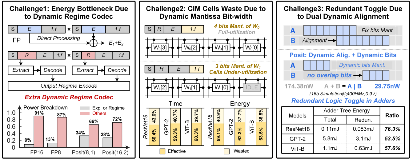
Fig. 3. Three challenges of designing energy-efficient POSIT-based CIM caused by the dynamic properties of POSIT data format.
