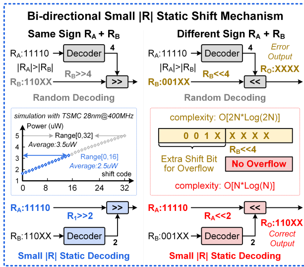
Fig. 6. Bi-directional small |R| static shift mechanism.
