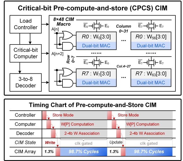
Fig. 10. Architecture and timing chart of CPCS CIM array.
