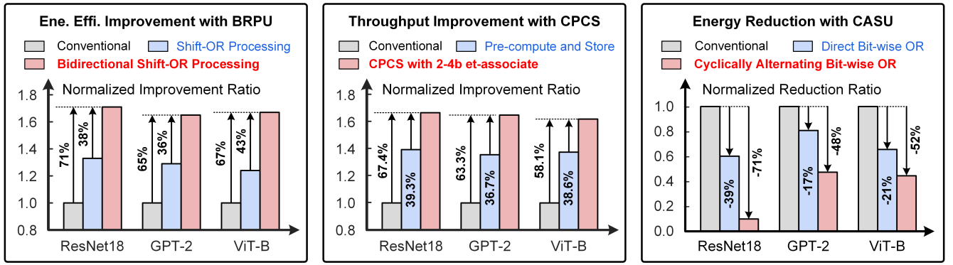
Fig. 17. Performance evaluations on the three key features.
