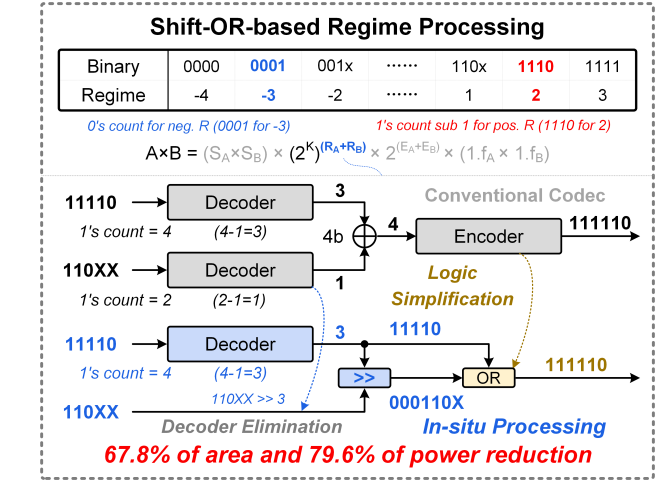
Fig. 5. Proposed shift-OR-based regime processing.
