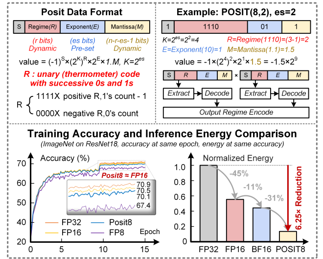
Fig. 2. Principle and performance of POSIT data format.
