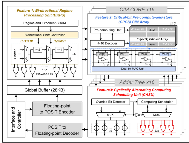
Fig. 4. Overall architecture of the proposed PD-CIM.
