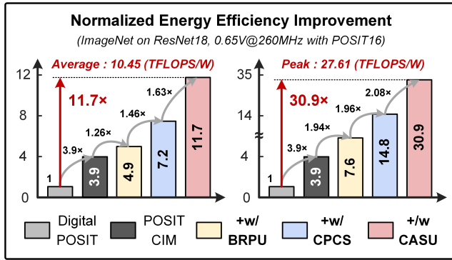
Fig. 18. Energy efficiency improvement with combined evaluation.
