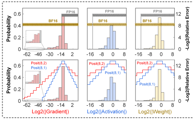
Fig. 1. Relative error comparisons of different data formats.
