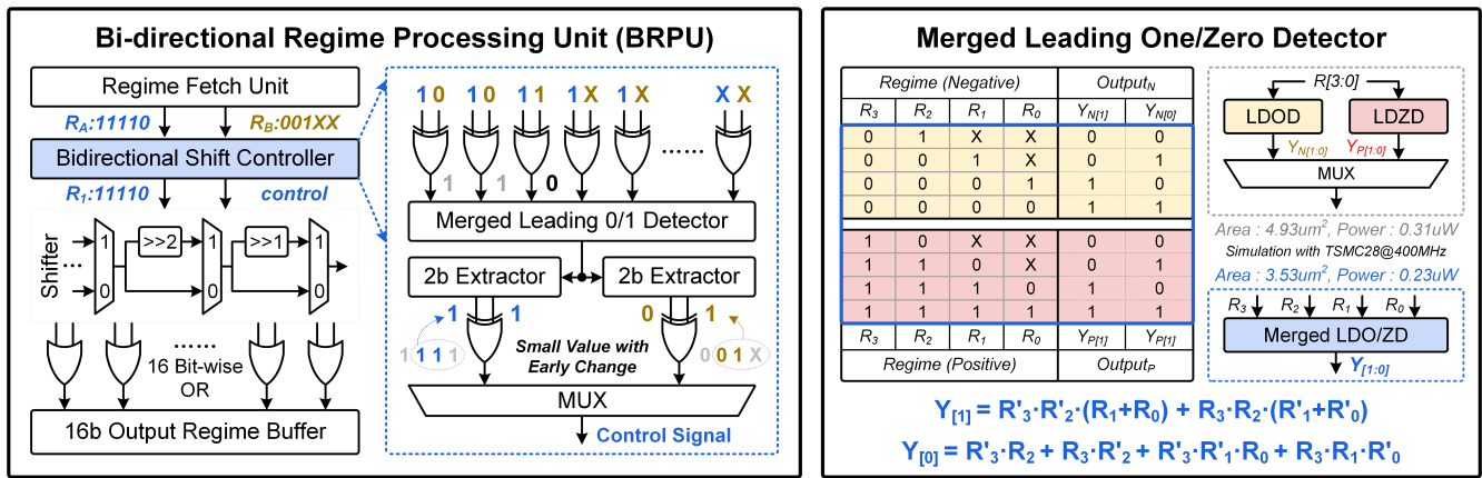
Fig. 7. Architecture and design details of BRPU.
