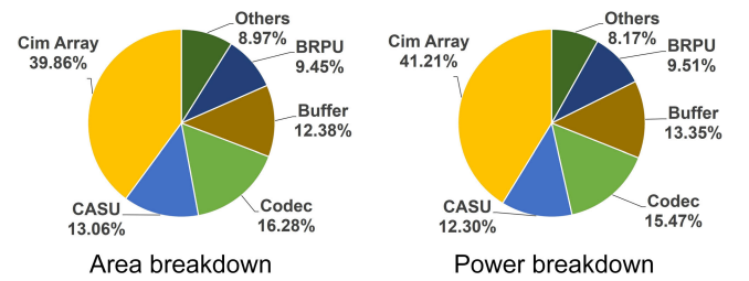
Fig. 15. Power and area breakdown of the proposed PD-CIM.
