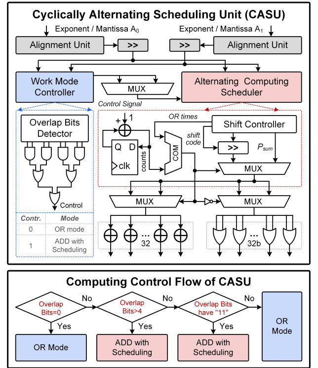
Fig. 13. Architecture and computing control flow of CASU.
