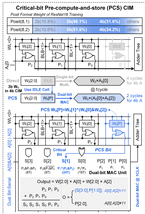
Fig. 8. Principle of CPCS mechanism.
