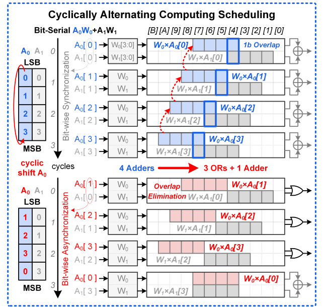
Fig. 12. OR-based accumulation with cyclical alternating scheduling.
