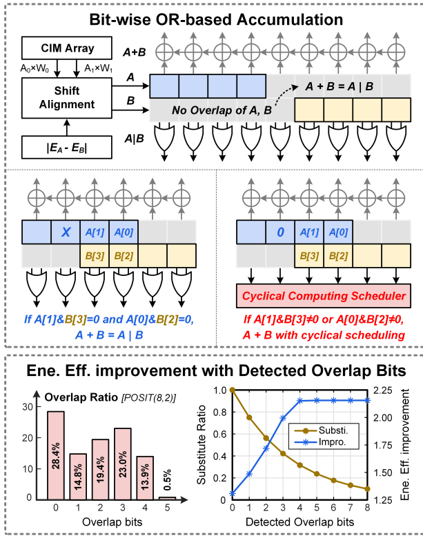
Fig. 11. OR-based accumulation for mantissas with no overlap bits.
