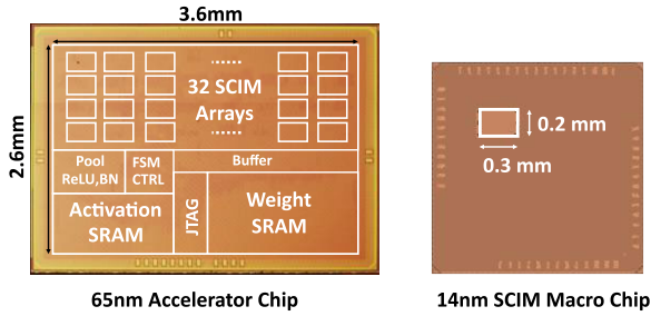
Fig. 14. 65- and 14-nm chip micrograph.
