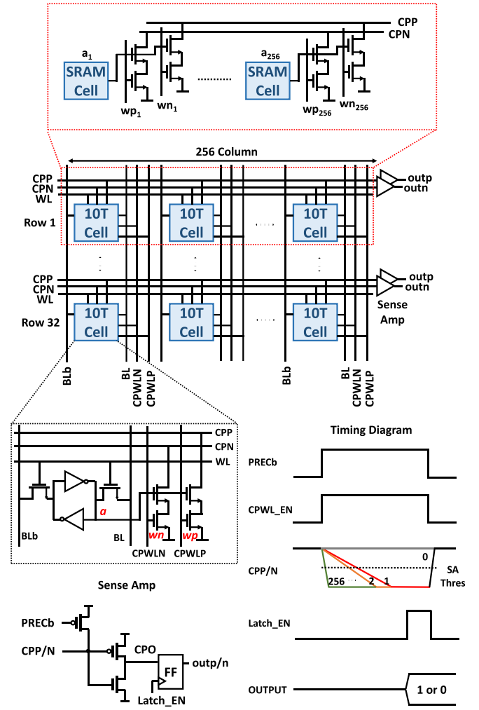
Fig. 7. SCIM bit cell array. Circuit implementation of 10T SCIM cell and sense amplifier. Timing diagram of a compute operation.
