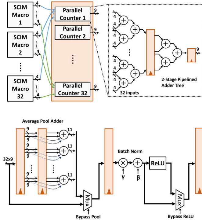
Fig. 12. Parallel counter for stochastic to binary conversion. Fixed-point domain processing.
