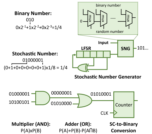
Fig. 2. Number representation and basic building blocks of SC.
