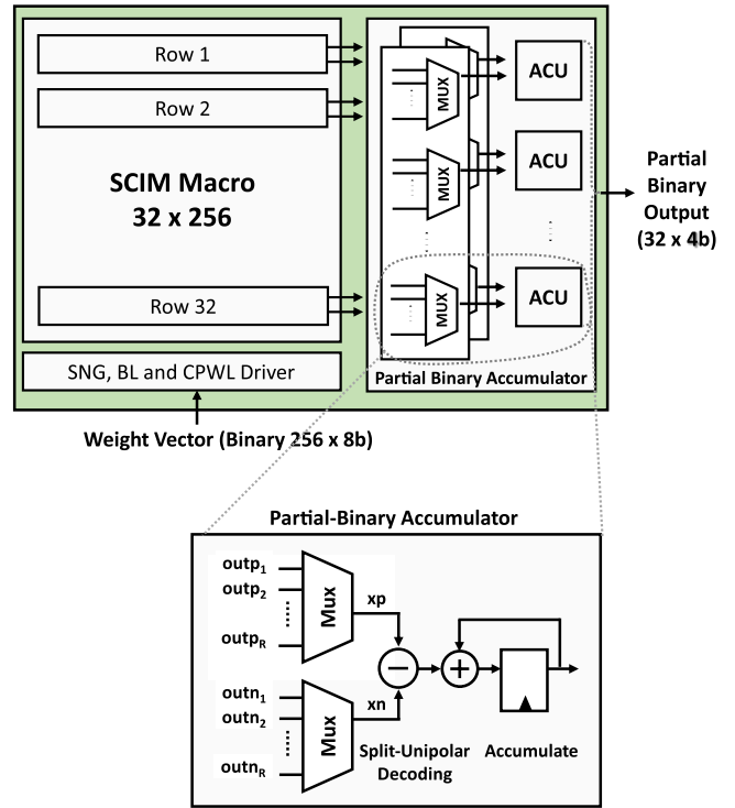
Fig. 10. Near-memory partial binary accumulator circuits.
