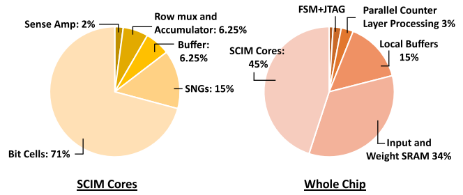
Fig. 16. Area breakdown of SCIM cores and whole chip.
