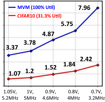
Fig. 17. Energy efficiency versus voltage.
