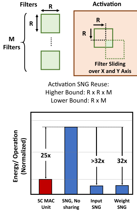
Fig. 6. Reuse of the stored activations (top). Energy cost of SNG with and without reuse (bottom).
