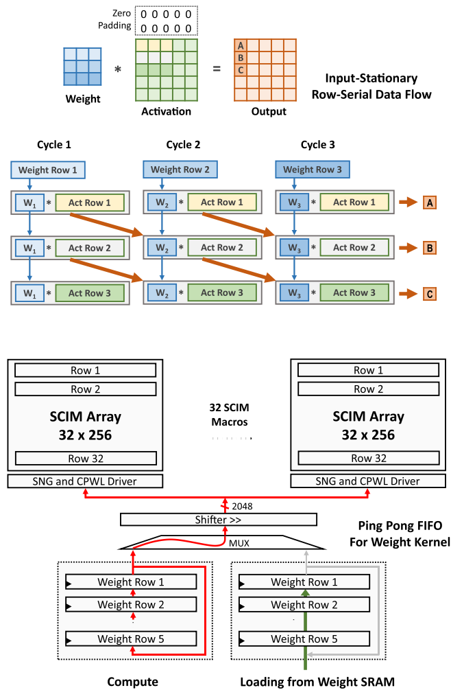
Fig. 11. Data flow of convolution. Ping-pong FIFO registers for weights.
