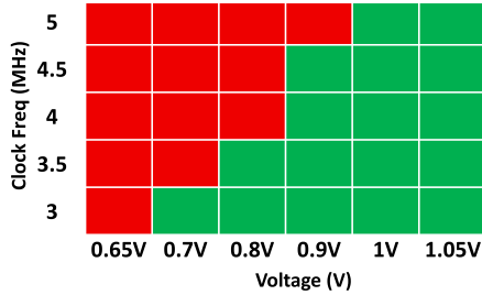
Fig. 15. 65-nm chip clock frequency versus voltage.
