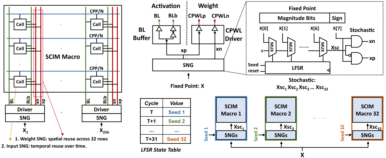
Fig. 5. SNG circuit. Data path of SNG for input and weight. Seed schedule for parallel SNGs.
