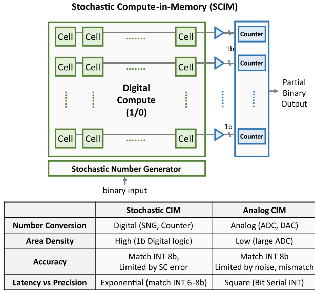
Fig. 1. High-level diagram of an SCIM macro, comparison between SCIM and analog CIM.
