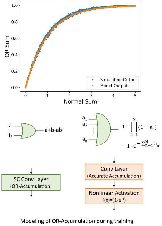
Fig. 13. OR accumulation's output versus accurate sum. Modeling of OR-accumulation during training.
