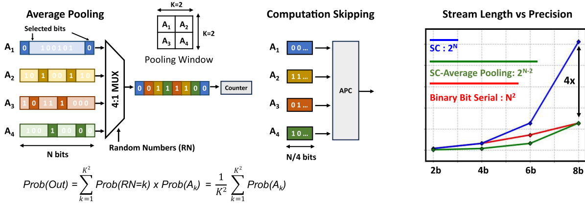
Fig. 8. Computation skipping of average pooling function. Stream length versus precision function.
