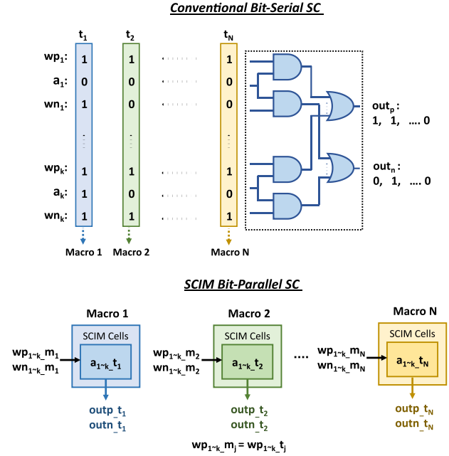
Fig. 4. Split-unipolar representation for inputs and weights. Bit-parallel processing and mapping to SCIM macros.
