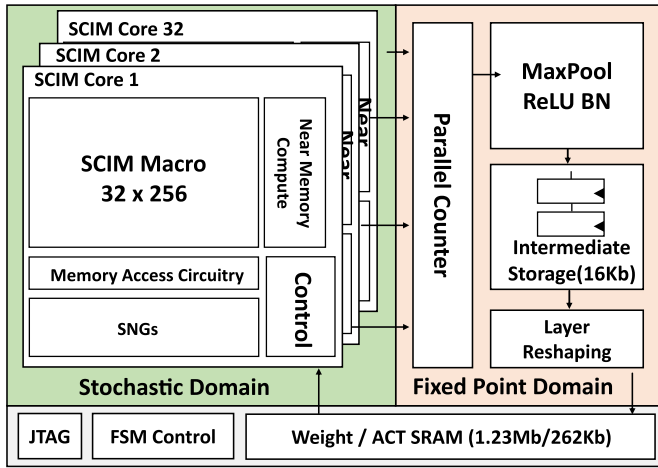
Fig. 3. Architecture of SCIM accelerator.
