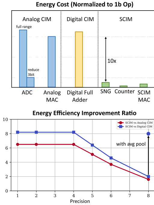
Fig. 9. Energy cost comparison of all components in CIM and SCIM macros normalized to 1-b Op. Energy efficiency improvement of SCIM over other CIMs versus precisions.
