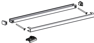
63-4422 Slide Assembly
