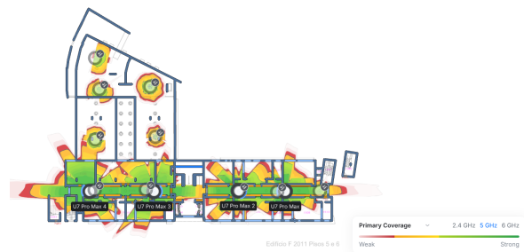
Figure 4: Heatmap (Piso 5) - 5GHz
