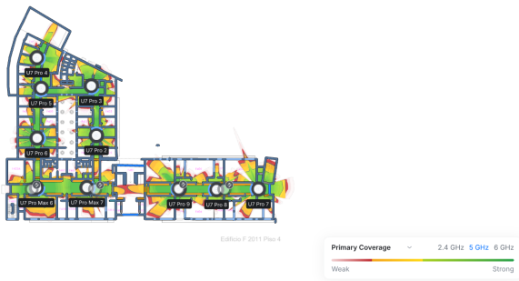
Figure 3: Heatmap (Piso 4) - 5GHz
