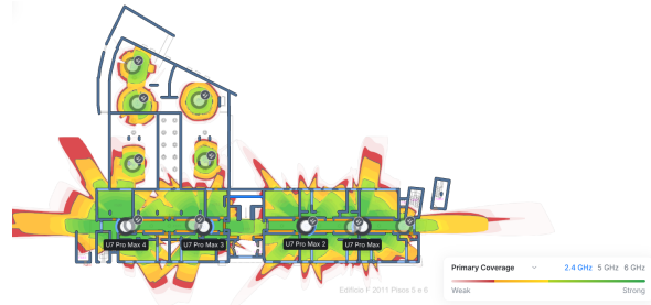
Figure 2: Heatmap (Piso 5) - 2.4GHz
