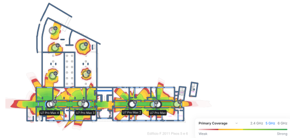
Figure 4: Heatmap (Piso 5) - 5GHz
