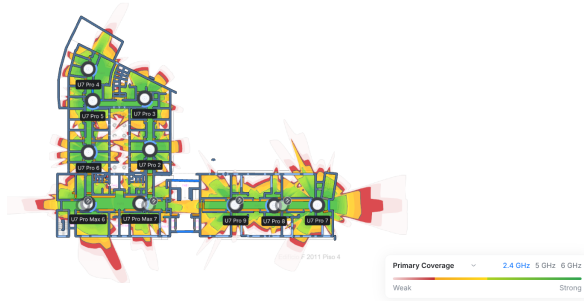
Figure 1: Heatmap (Piso 4) - 2.4GHz
