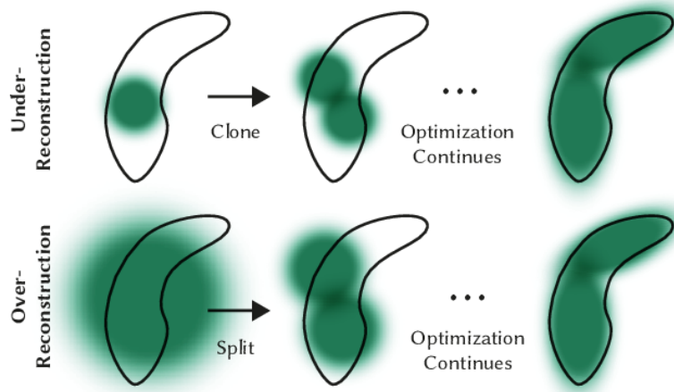
Figure 2: Adaptive Density Control situations for over- and under-reconstruction portraying cloning and splitting (from [11])
