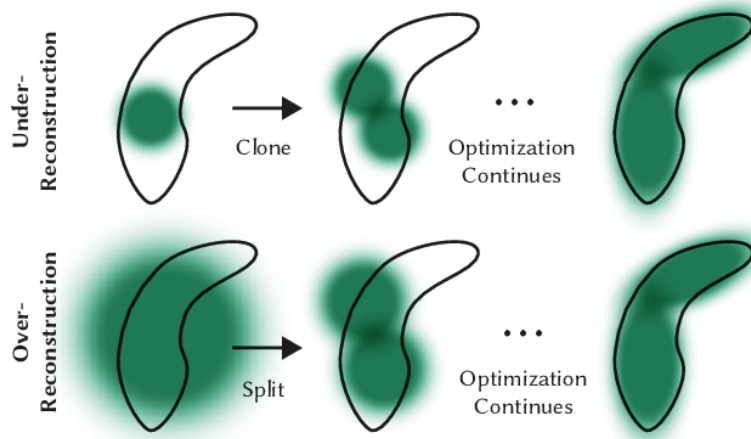
Figure 2: Adaptive Density Control situations for over- and under-reconstruction portraying cloning and splitting (from [10])
