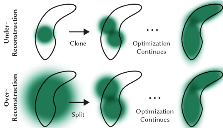
Figure 2: Adaptive Density Control situations for over- and under-reconstruction portraying cloning and splitting (taken from [12]).
