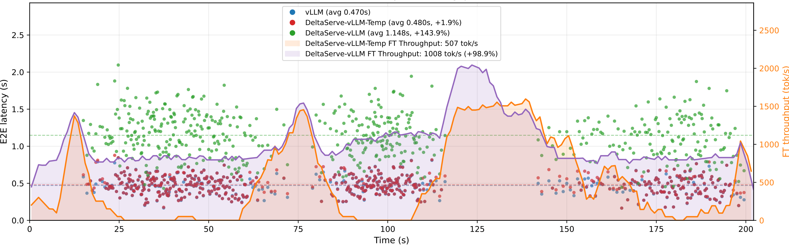
5090 — E2E latency &amp; FT throughput
