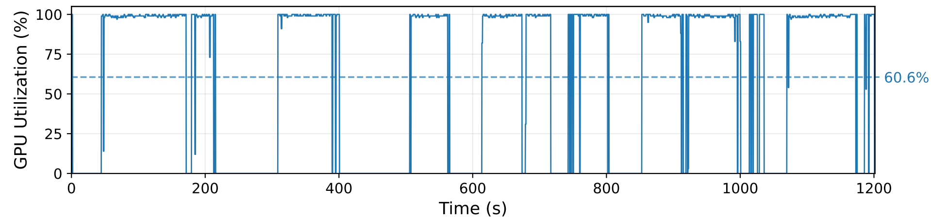
GPU Utilization Under Production Workload
