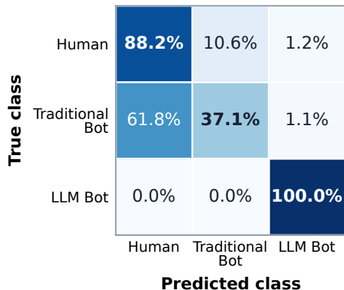
(a) Twibot22 - BotDMM
