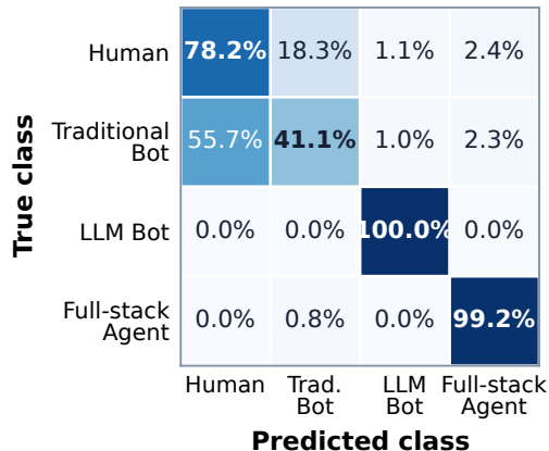
(c) Quadbot - BotDMM
