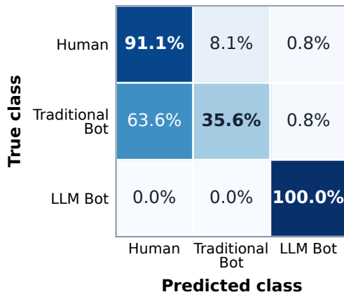
(b) Twibot22 - CBAF-Net
