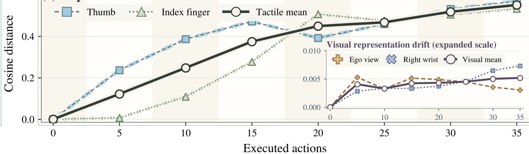
(c) Representation drift over the action horizon
