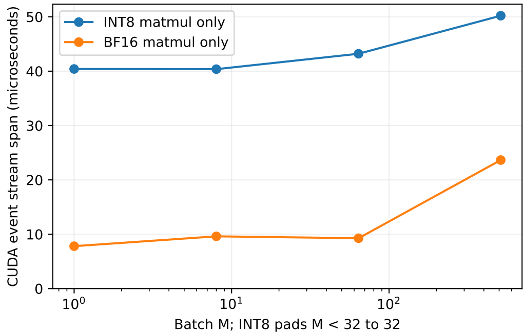
RTX PRO 6000: checkpoint expert; same INT8 weights and activation quantization
