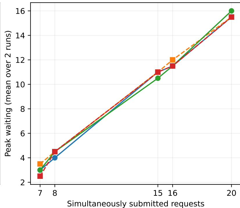
Online FP8 weights / 8 GiB KV / 7,239 input tokens / shared GPU
