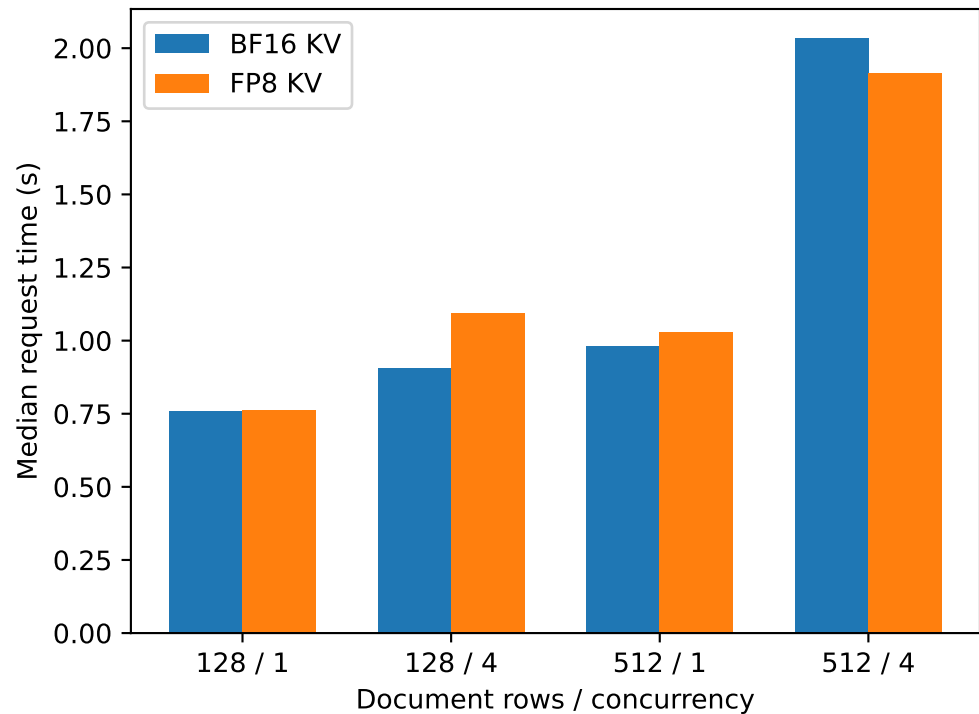
Online FP8 weights; 8 GiB KV budget; shared RTX PRO 6000
