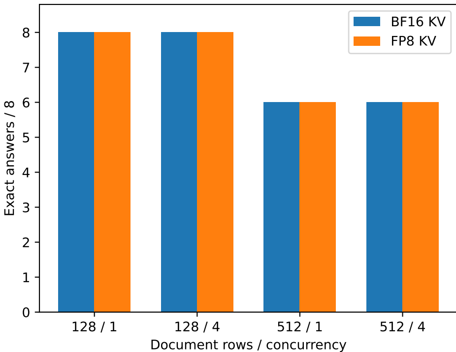
Online FP8 weights; 8 GiB KV budget; shared RTX PRO 6000
