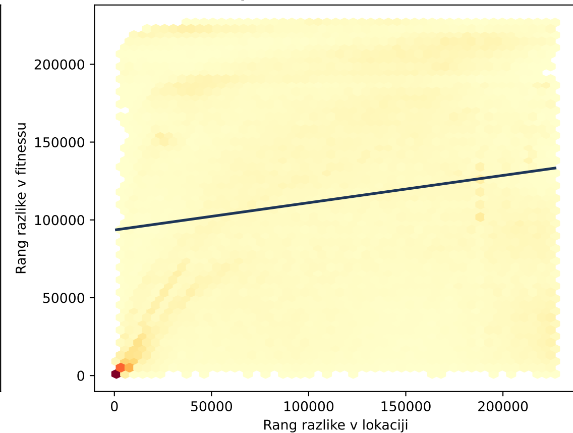
Dimenzija 10 ( \rho = 0.18 , n = 226800 )
