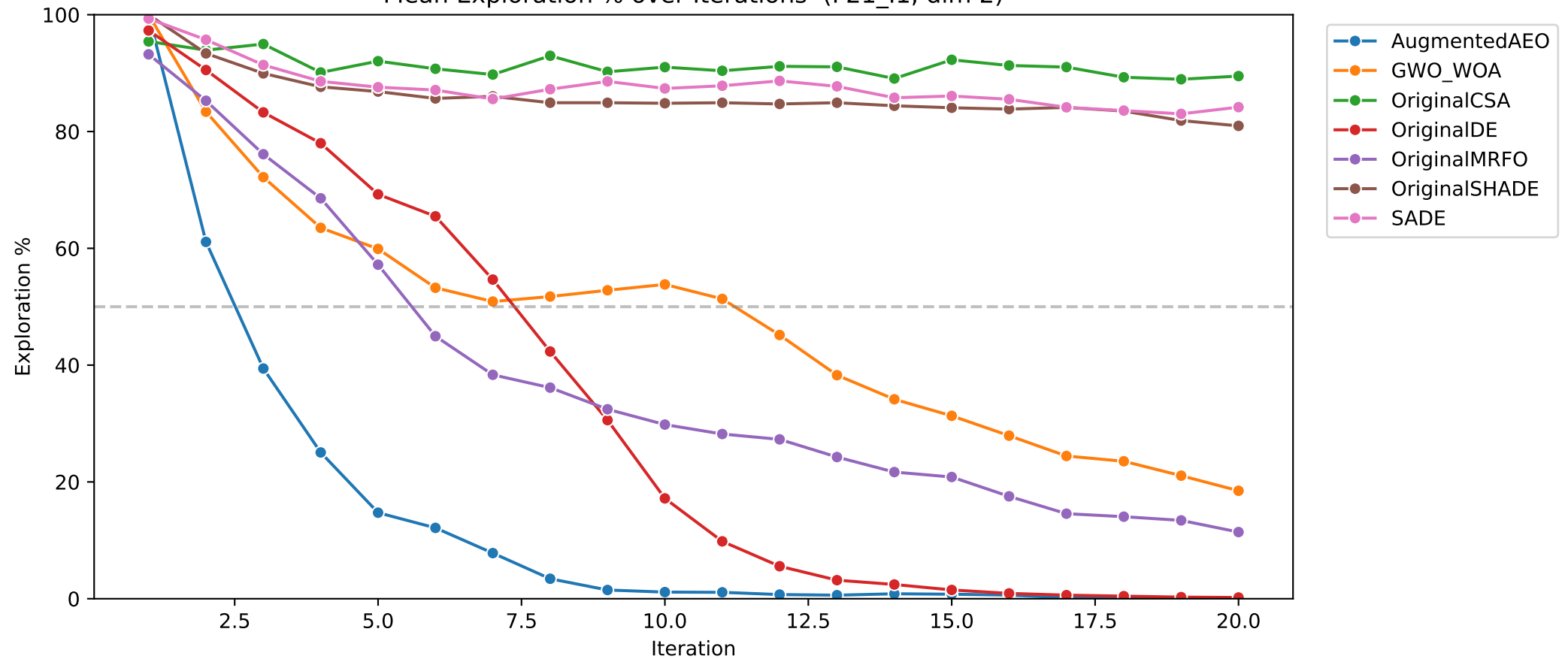
Mean Exploration % over Iterations (F21_I1, dim 2)
