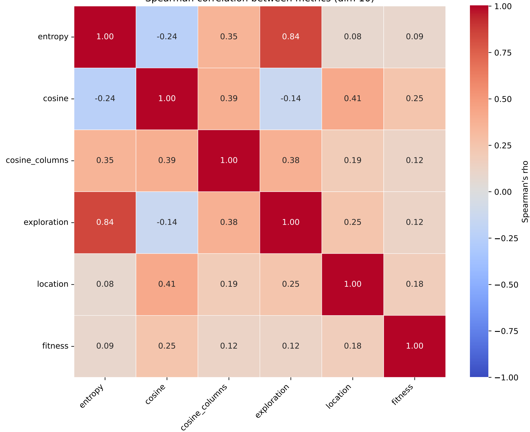
Spearman correlation between metrics (dim 10)
