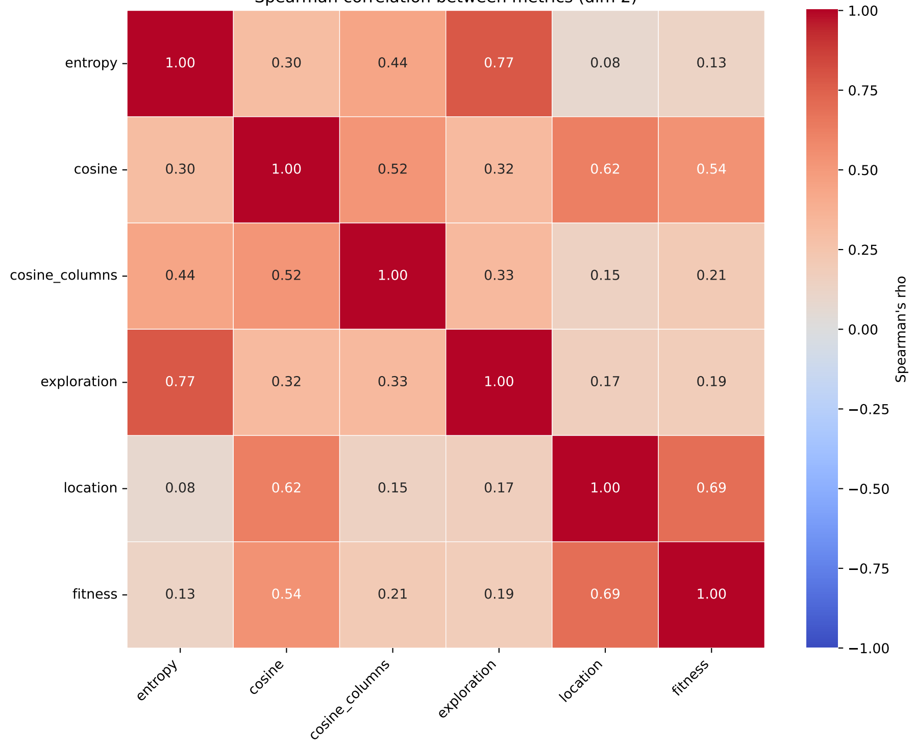
Spearman correlation between metrics (dim 2)
