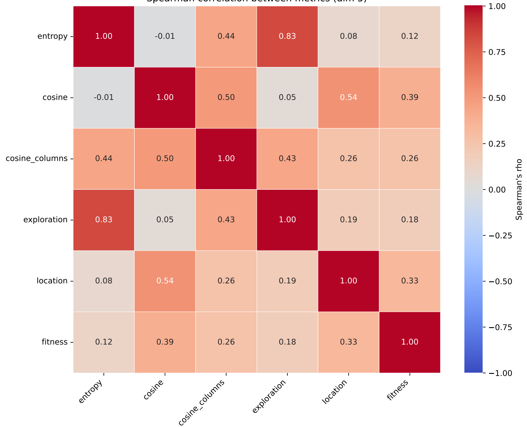
Spearman correlation between metrics (dim 5)
