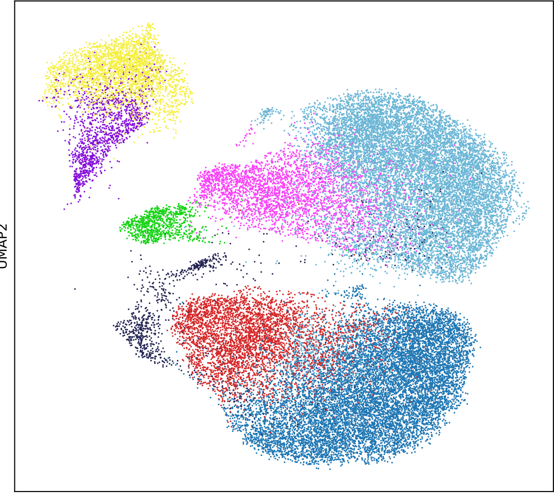
NucSeq
