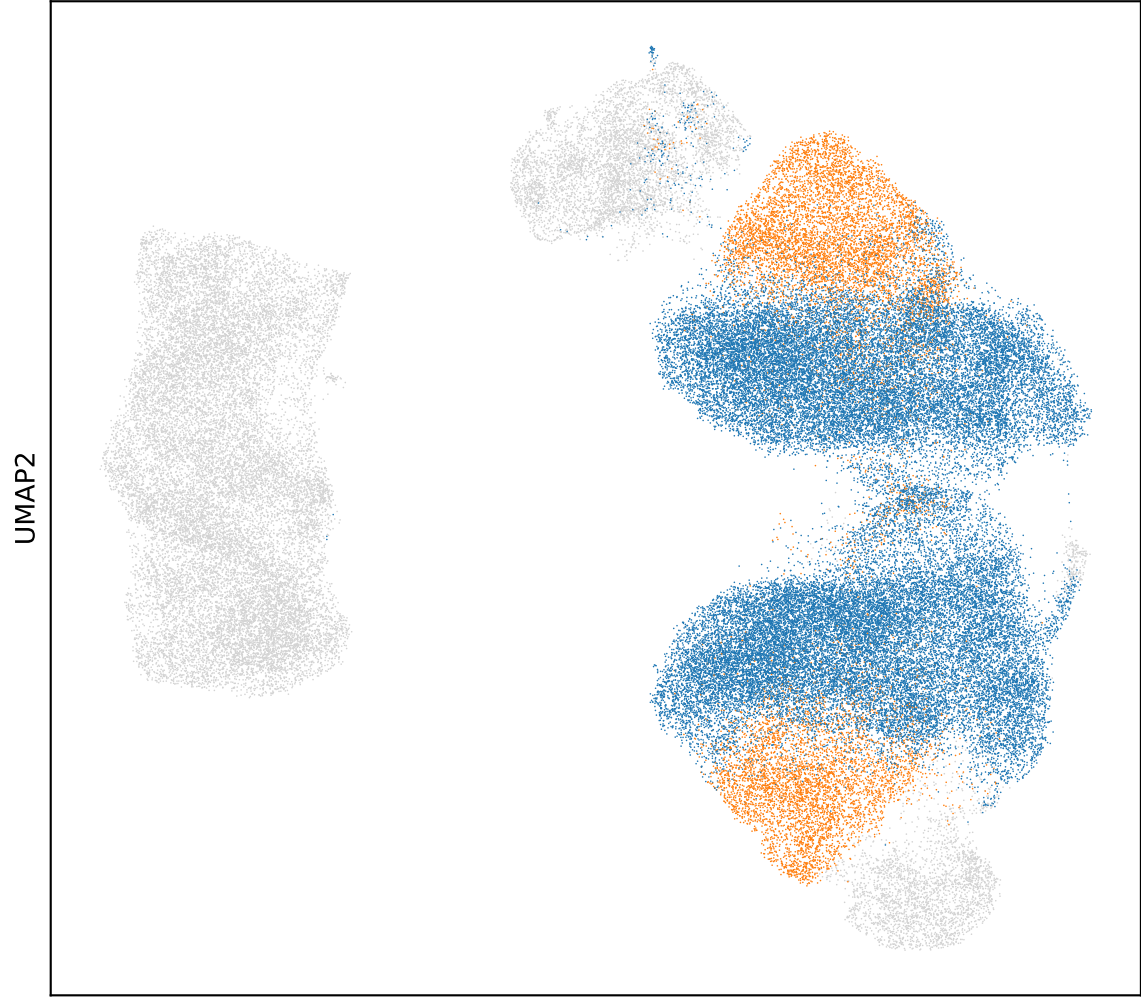
matrix_vs_patch
