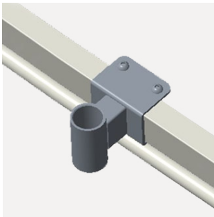
Trapeze Bracket
